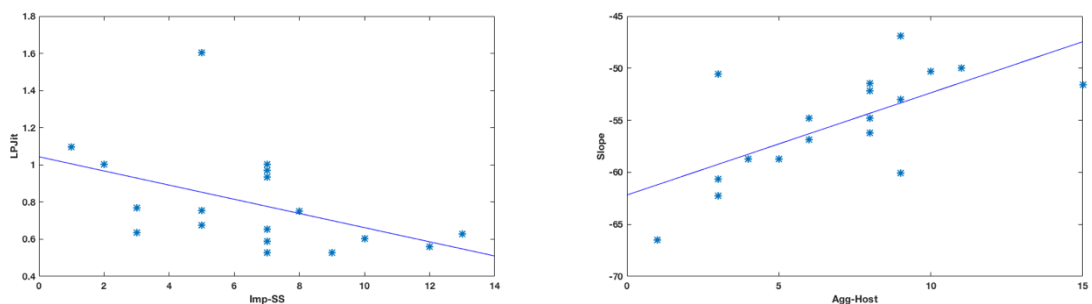
Figure 4. TAT task. Left: scatter plot of LPJit and Imp-SS. ( \rho = -0.60 ). Right: Slope and Agg-Host ( \rho = 0.66 ). \rho refers to the Spearman's correlation coefficient between the corresponding speech feature and personality score across 18 subjects
