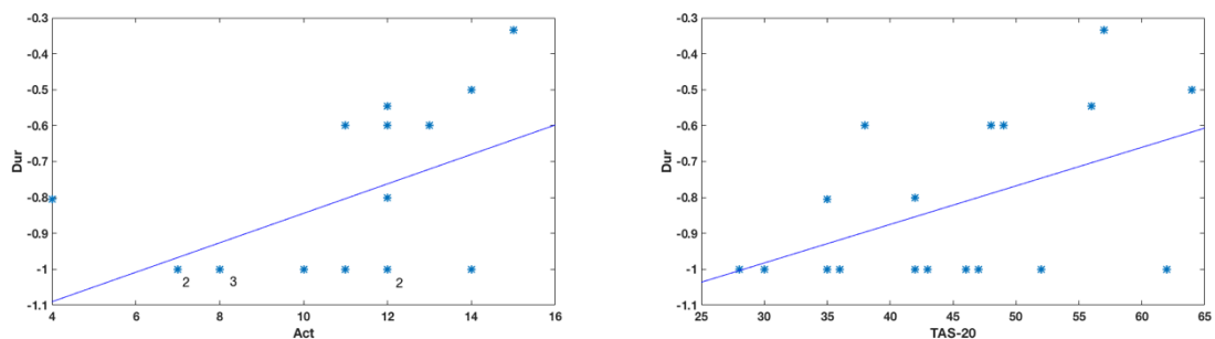
Figure 6. TAT task. Left: scatter plot of Dur vs Act ( \rho=0.56 ). Right: scatter plot of Dur vs TAS-20 ( \rho=0.48 ). \rho refers to the Spearman's correlation coefficient between the corresponding speech feature and personality score across 18 subjects. The multiplicity of coinciding measurements is shown.
