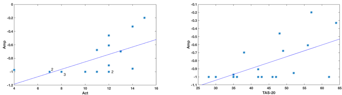
Figure 5. TAT task. Left: scatter plot of Amp vs Act ( \rho=0.67 ). Right: scatter plot of Amp vs TAS-20 ( \rho=0.56 ). \rho refers to the Spearman's correlation coefficient between the corresponding speech feature and personality score across 18 subjects. The multiplicity of coinciding measurements is shown.
