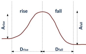
Figure 2. Parameters of the Tilt Model.
