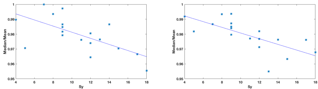
Figure 3. Reading task: scatter plot of Median/Mean vs Sy. Left: Rd1 ( \rho = -0.66 ). Right: Rd2 ( \rho = -0.82 ). \rho refers to the Spearman's correlation coefficient between the corresponding speech feature and personality score across 18 subjects.
