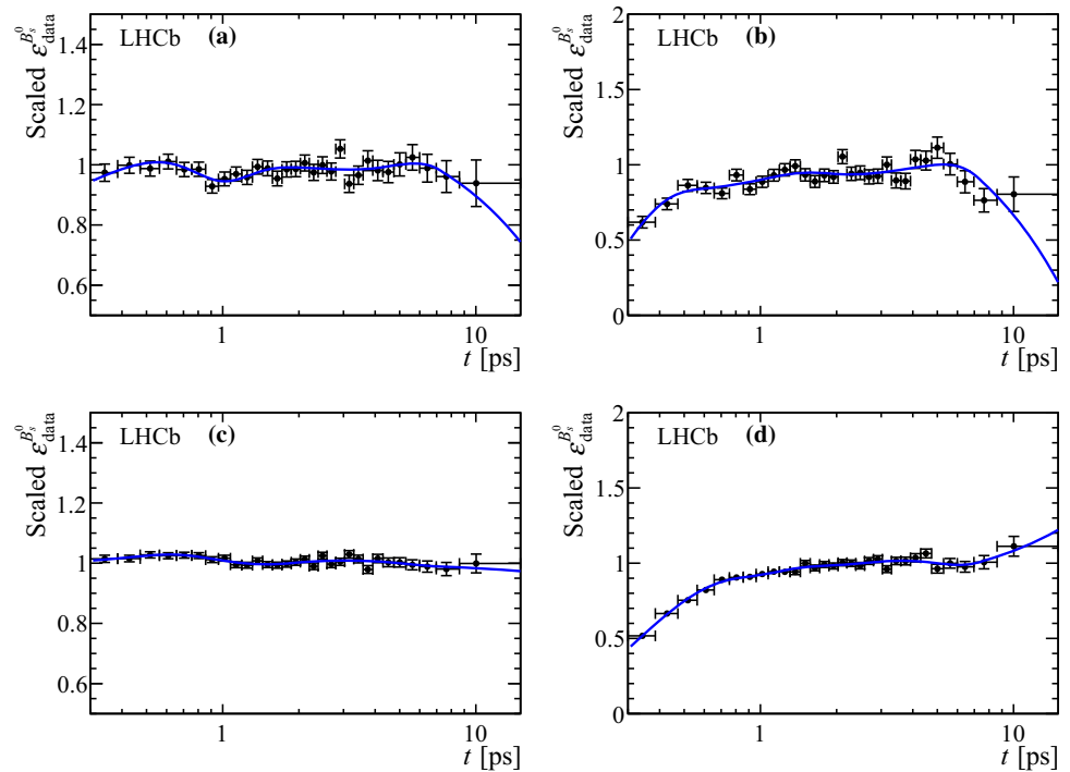
Fig. 5 Decay-time efficiency for the a 2015 unbiased, b 2015 biased, c 2016 unbiased and d 2016 biased B_s^0 \rightarrow J/\psi \phi sample. The cubic-spline function described in the text is shown by the blue line. For comparison, the black points show the efficiency when computed using histograms for each of the input component efficiencies
