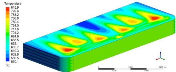
Fig. 3. WCLL 2018 OB equatorial breeding cell: Eurofer and Tungsten domain temperature
