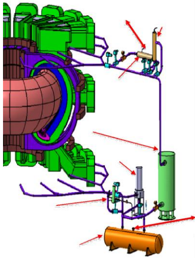
Fig. 4. Layout of a PbLi loop for WCLL BB inboard segments.
