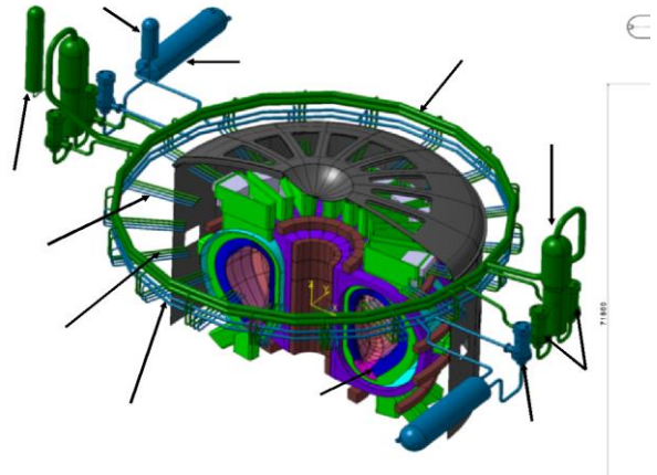
Fig. 5. Layout of the FW and BZ PHTS.
