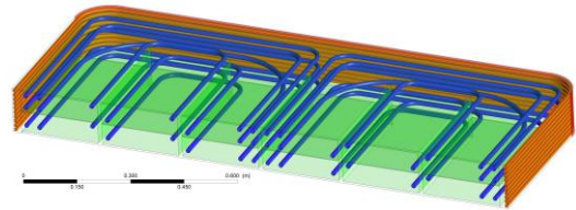
Fig. 2. WCLL 2018 OB equatorial breeding cell geometry.
