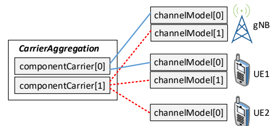
Figure 11: Example of CA configuration.
