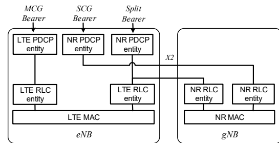
Figure 6: Interactions between eNB and gNB in an ENDC deployment.
