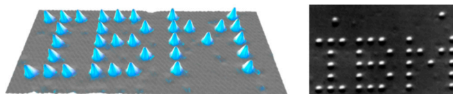
Figure 7. 35 Xenon atoms positioned on a nickel (110) substrate using a STM to form IBM logo. Reproduced with permission from reference [23].
