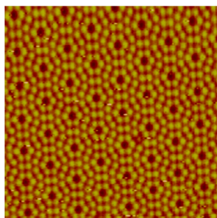
Figure 6. STM image of the Si(111)- 7 \times 7 reconstructed surface showing atomic scale resolution of the top-most layer of silicon atoms. Reproduced with permission from reference [22].
