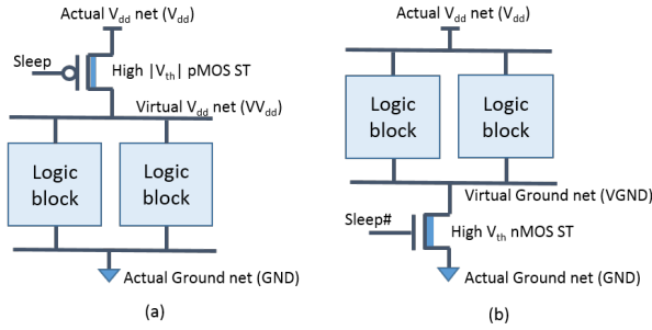
Fig. 1. Power-gating approaches: (a) header pMOS ST; (b) footer nMOS ST.
