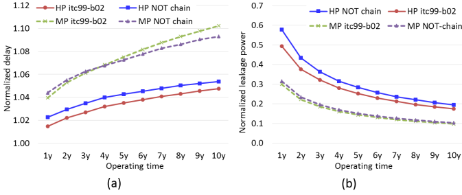
Fig. 8. Profile over time of (a) normalized propagation delay (normalization factors: \tau_{wc,b02}(t0) = 59.63ps ; \tau_{wc,NOT}(t0) = 118.3ps ) and (b) normalized power leakage (normalization factors: EP_{leak0}(b02)=62.1pW , EP_{leak0}(NOT)=32.2pW ).
