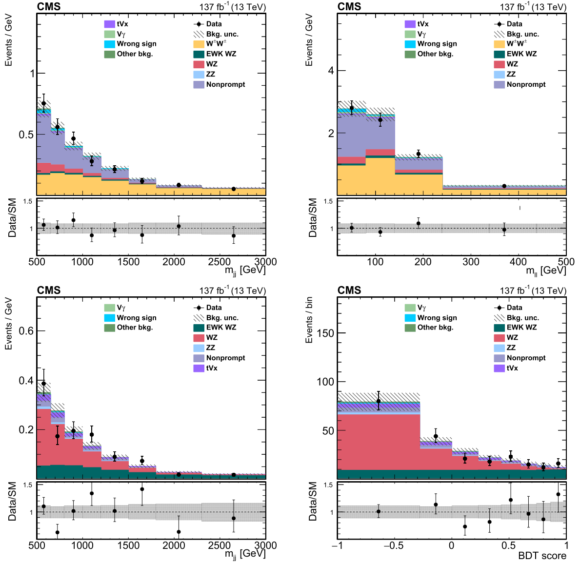
Fig. 3. Distributions of m_{jj} (upper left) and m_{\ell\ell} (upper right) in the W^\pm W^\pm SR, and the distributions of m_{jj} (lower left) and BDT score (lower right) in the WZ SR. The predicted yields are shown with their best fit normalizations from the simultaneous fit. Vertical bars on data points represent the statistical uncertainty in the data. The contribution of the QCD W^\pm W^\pm process is included together with the EW W^\pm W^\pm process. The histograms for tVx backgrounds include the contributions from t\bar{t}V and tZq processes. The histograms for other backgrounds include the contributions from double parton scattering and VVV processes. The histograms for wrong-sign background include the contributions from oppositely charged dilepton final states from t\bar{t} , tW , W^+W^- , and Drell-Yan processes. The overflow is included in the last bin. The bottom panel in each figure shows the ratio of the number of events observed in data to that of the total SM prediction. The gray bands represent the uncertainties in the predicted yields.
