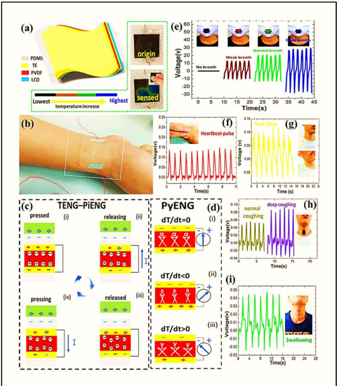
Figure 4.1: (a) A schematic diagram of the transparent HBNG with a thermochromic liquid crystal (LCD) film integrated between the transparent electrodes and PDMS. The LCD film changes color with increasing temperature, from black to blue, so that the entire device can be used as a visual thermometer. (b) A photograph showing the transparency of the HBNG attached on skin. The working mechanisms of (c) the integrated triboelectric nanogenerator and piezoelectric nanogenerator (TENG-PiENG) and (d) the pyroelectric nanogenerator. (e) When attached to a respirator, the HBNG's voltage output's magnitude corresponded with the strength of the breath. The HBNG was also attached to the wrist, the front of neck, and the side of the neck and distinct voltage outputs for (f) a heartbeat pulse, (g) neck tilting, (h) different intensity coughing, and (i) swallowing were recorded.
