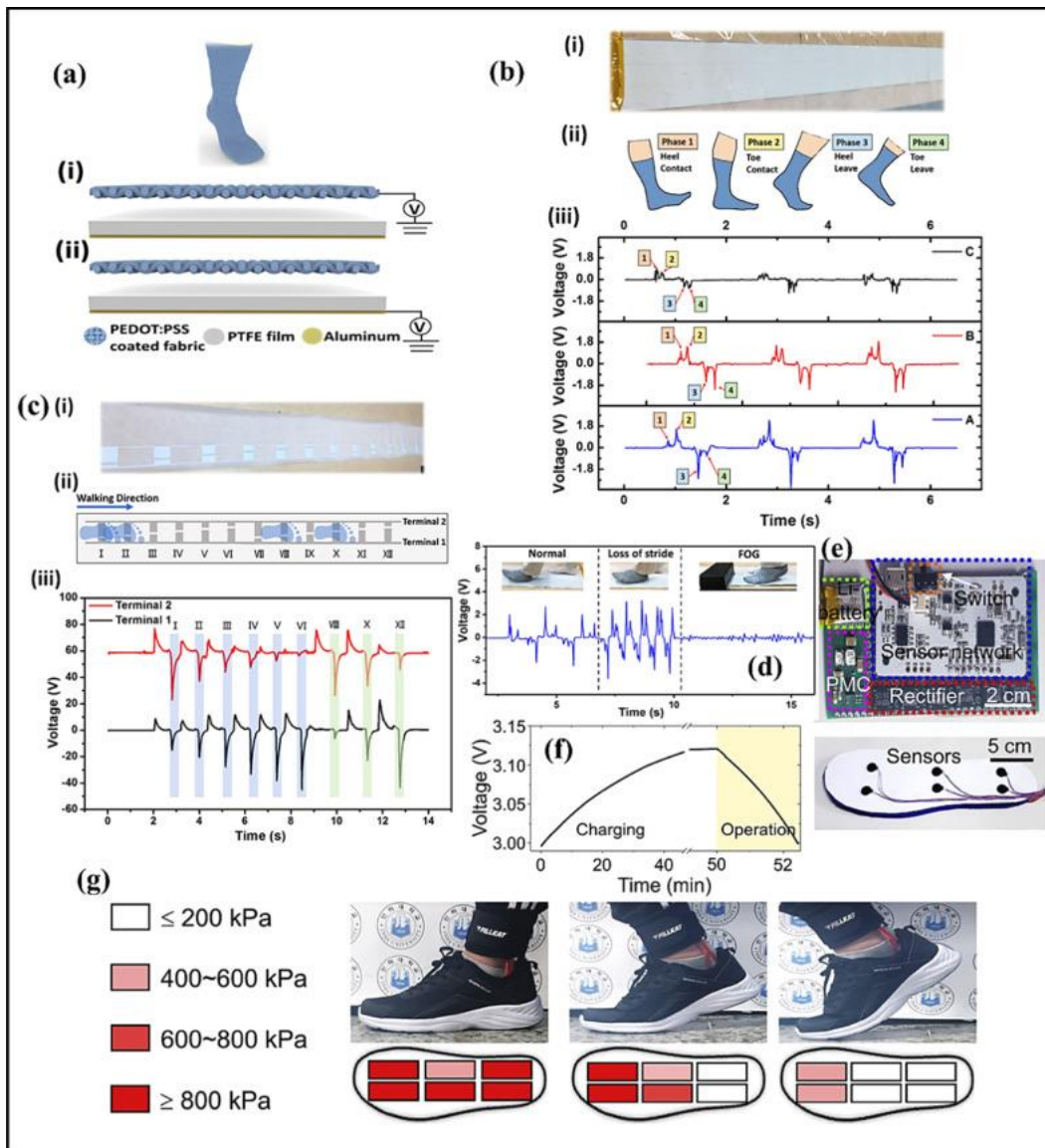
Figure 4.4: (a) A schematic diagram of the modified sock and the PTFE film with aluminium electrodes (i, ii). The device has two modes of electrical connections, the (i) sock connection and the (ii) Al/PTFE connection. (b) The device can help analyze footsteps. (i) A photograph of the PTFE laid on the floor like a carpet. The phases of a footstep (ii) can be reflected by the (iii) sock
