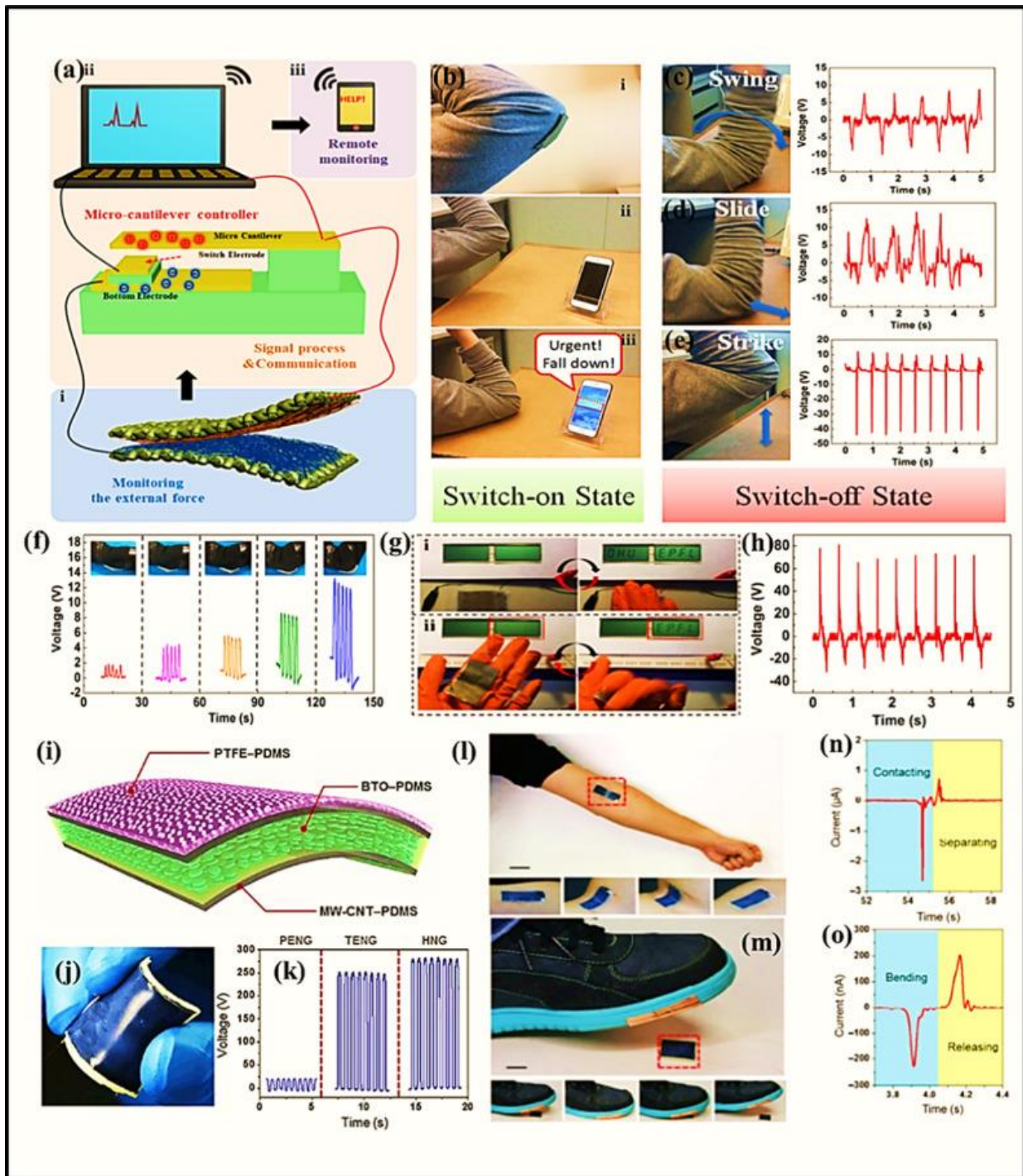
Fig. 5.1: (a) An illustration of a fall alert system by fiber based HBNG. The device was tested attached to the elbow (b), and a simulated fall by dropping the elbow against the table (b ii) resulted in an emergency message (iii). Additionally, the device can also be used in energy harvesting while the electrical output does not reach the threshold, and the outputs of common motions like a swing (c), slide (d), and strike (e) are shown. (f) Different voltage outputs for different bending angles from 101^\circ to 146^\circ for the HBNG when attached to the elbow. The device was used to power LCDs with tapping (g i) and with folding (g ii). The voltage output with \sim 2 Hz frequency hand tapping reached 78 V (h). (i) A schematic diagram of a HBNG fabricated using multilayered nanocomposite materials with a PTFE nanoparticle and PDMS matrix top layer. The device is flexible and can be bent (j). The output was recorded (k), and the hybrid nanogenerator output (HNG) exceeded both the TENG and PENG outputs. (l) The hybrid nanogenerator used to harvest energy from the flexion
