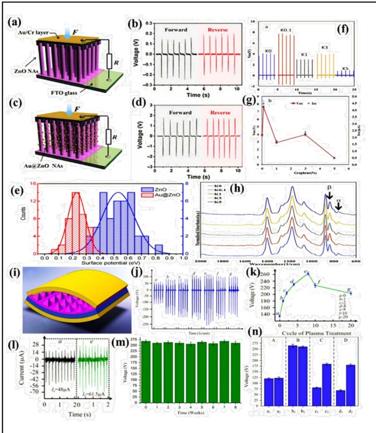
Figure 5.2: schematic diagram of (a) ZnO NA-based PENG without Au, (b) along with its output voltage, and (c) ZnO NA-based PENG with Au, (d) along with a significantly higher voltage. The distribution of surface potential for the device with and without gold, (e) shows average surface potential for ZnO with Au. (f) Open circuit voltage ( V_{oc} ) for a nanofiber sample with no graphene (KO), 0.1 wt% graphene (K0.1), 1 wt% graphene (K1), 3 wt% graphene (K3), and 5 wt% graphene
