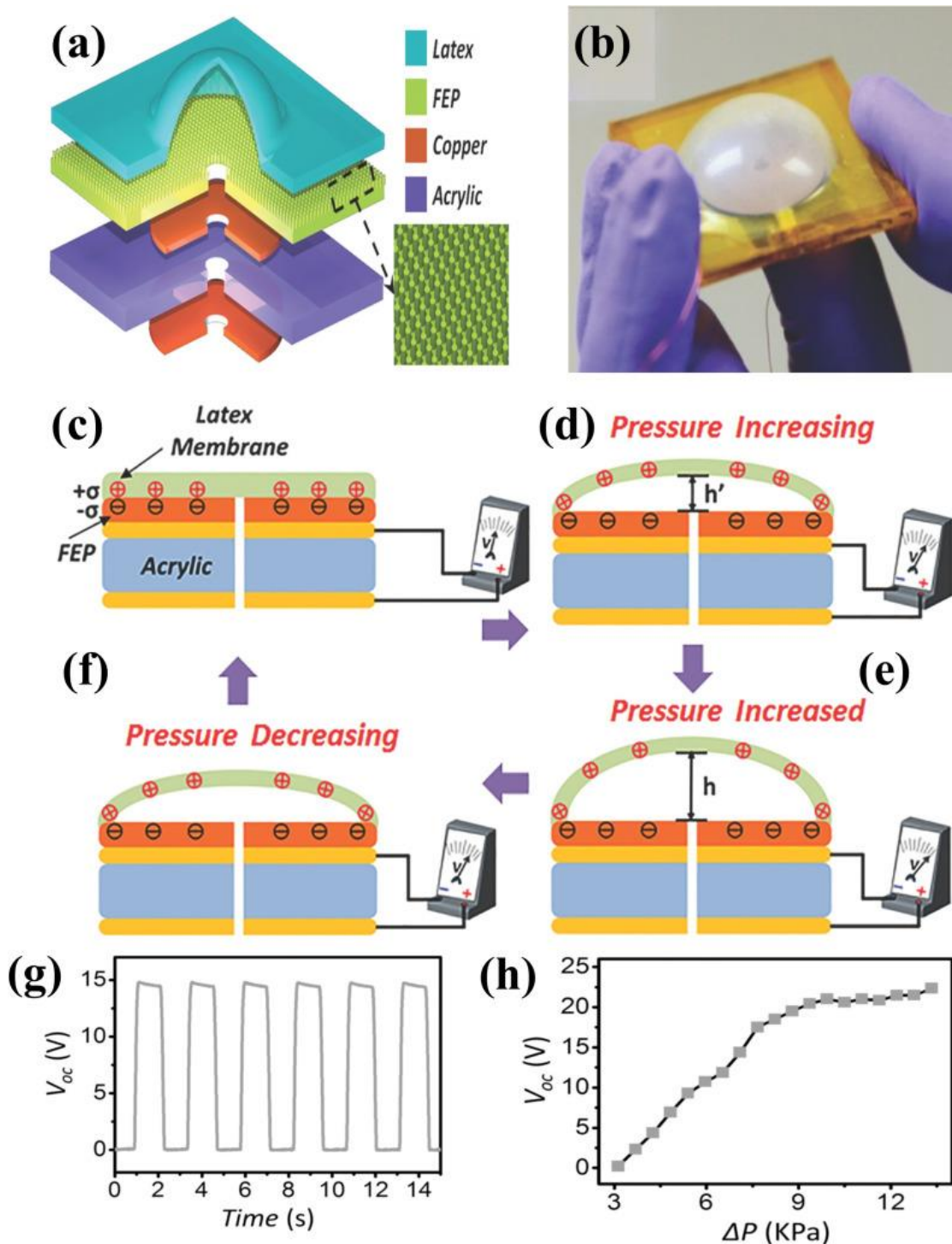
Figure 2.2: (a) Schematic of the M-TES, (b) M-TES with the latex membrane swelling, Working principle of the M-TES in open-circuit condition- (c) The initial state, (d) separation of the charged surfaces, (e) fully separated position and (f) the two surfaces are approaching to each other, (g) V_{oc} of the M-TES when air pressure increases. (h) Dependence of V_{oc} on the increased air pressure.
