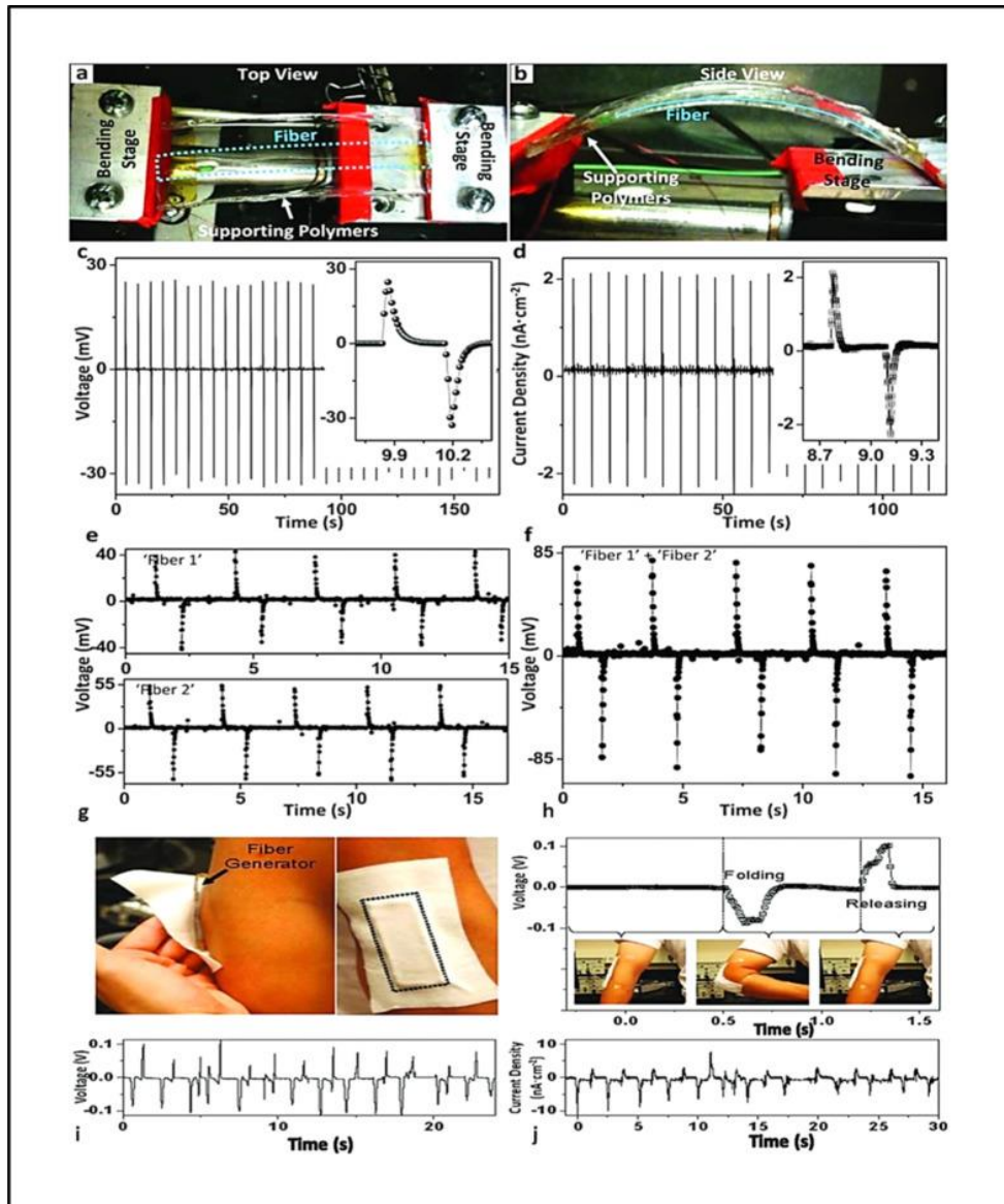
Figure 3.2: and electrical outputs of hybrid-fiber nanogenerators. Top-view (a) and side-view (b) of a hybrid-fiber device attached to a PS substrate and covered in PDMS for uniform stress, on a bending stage. Open-circuit output voltage (c) and closed-circuit output current density of a fiber device (d) under a strain of \sim 0.1\% . Open-circuit voltage outputs (e) of two different fiber devices, labeled ‘Fiber 1’ and ‘Fiber 2’, under a strain of \sim 0.1\% . Open-circuit voltage output of Fiber 1 and Fiber 2 (f) connected in series under a strain of \sim 0.1\% and at a strain rate of \sim 2.3\% \text{ s}^{-1} . Photographs of the hybrid-fiber device (g), and PDMS/PS were attached in the same way and for the same reason as in (a). Open-circuit voltage output (h) of a fiber device from the flexion and extension (folding and
