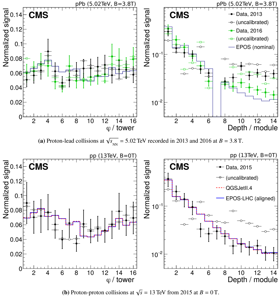
Figure 30. CASTOR signal response in calibrated (filled symbols) and uncalibrated (open symbols) data compared to the detector simulations (histograms), projected into the azimuthal (left) and longitudinal (right) direction. Upper: comparison of minimum-bias pPb collision data recorded in 2013 and 2016 with the EPOS-LHC simulations (with the nominal MC geometry). The impact of the magnetic field around module 7 is clearly visible. Lower: comparison of the minimum-bias pp collision data at \sqrt{s} = 13 TeV to the QGSJETII and EPOS-LHC (with geometry tuned to the 2015 data alignment) simulations. The CMS magnet was off while taking those data. The uncertainties of the calibrated data in all plots are statistical only, and originate almost entirely from the limited beam halo statistics for intercalibration. There is an additional scaling factor of 1.25 on the uncertainties of the calibrated data, as discussed in the text.
