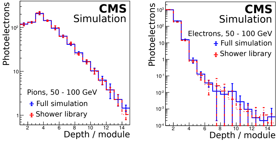
Figure 28. Comparison of the full (blue histogram) and fast (red histogram) simulation responses (number of photoelectrons as a function of detector depth) for charged pion (left) and electron (right) showers penetrating CASTOR with energies from 50 to 100 GeV. Error bars around data points indicate statistical uncertainties.
