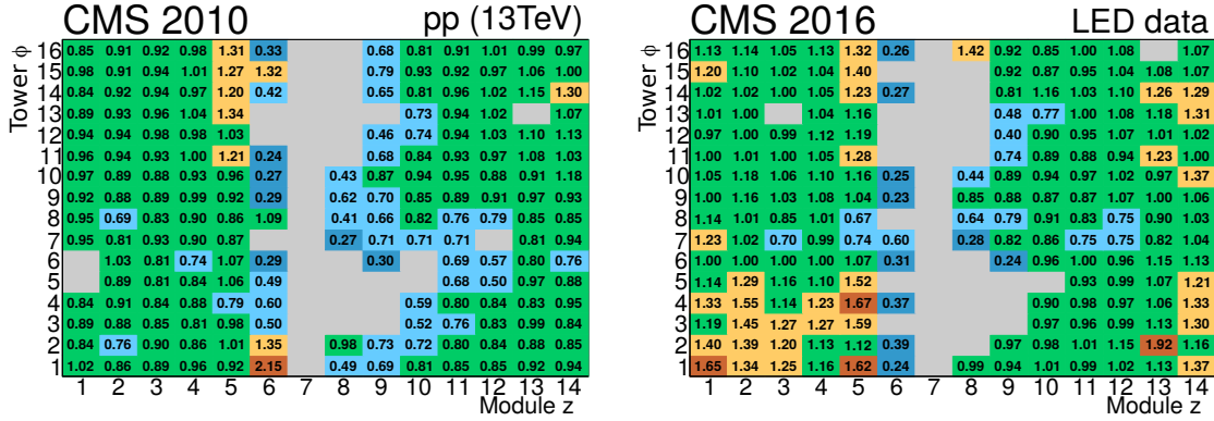
Figure 6. Impact of the CMS magnet on the signals observed in the CASTOR calorimeter in the ( z, \phi ) plane for 2010 pp minimum-bias (left) and 2016 LED pulser (right) data. The numerical values at each bin correspond to the ratio of signals measured at 3.8 T over those at 0 T. The channels in gray have normalized signals below 0.2, or are excluded for technical reasons.
