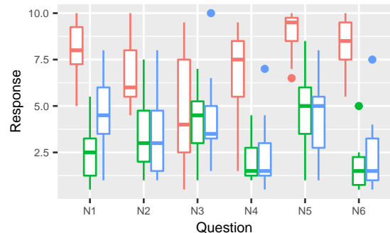
Fig. 5. NASA-TLX scores. Results considering a 21-points scale between 0 and 10, split per question and condition: in red NGc, green Vc, and blue Hc. All participants together.
