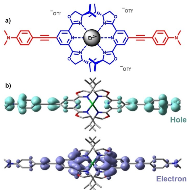
Figure 1. a) Structure of [Er( R,R )-L 2 ]:3OTf. b) Hole and electron distributions for the first excited state calculated for [Lu( R,R )-L 2 ] 3+ at CAM-B3LYP/def2-SVP/DZP[Lu]//B3LYP-D3B/def2-SVP/DZP[Lu] level; isovalue 0.0008.
