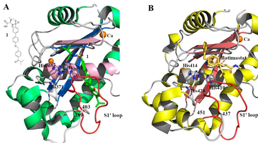
Figure 3. Structure of the aggrecanase Mp domain in complex with hydroxamate inhibitors. (A) Crystal structure of ADAMTS4 (PDB 2RJP) complexed with compound 1; the \beta strand and \alpha helix of the active site are shown in light pink, the S1' loop in red. (B) Crystal structure of ADAMTS5 (PDB 2RJQ) in complex with Batimastat. The S1' loop is shown in red. Zinc and calcium ion are colored in gray and in orange, respectively.
