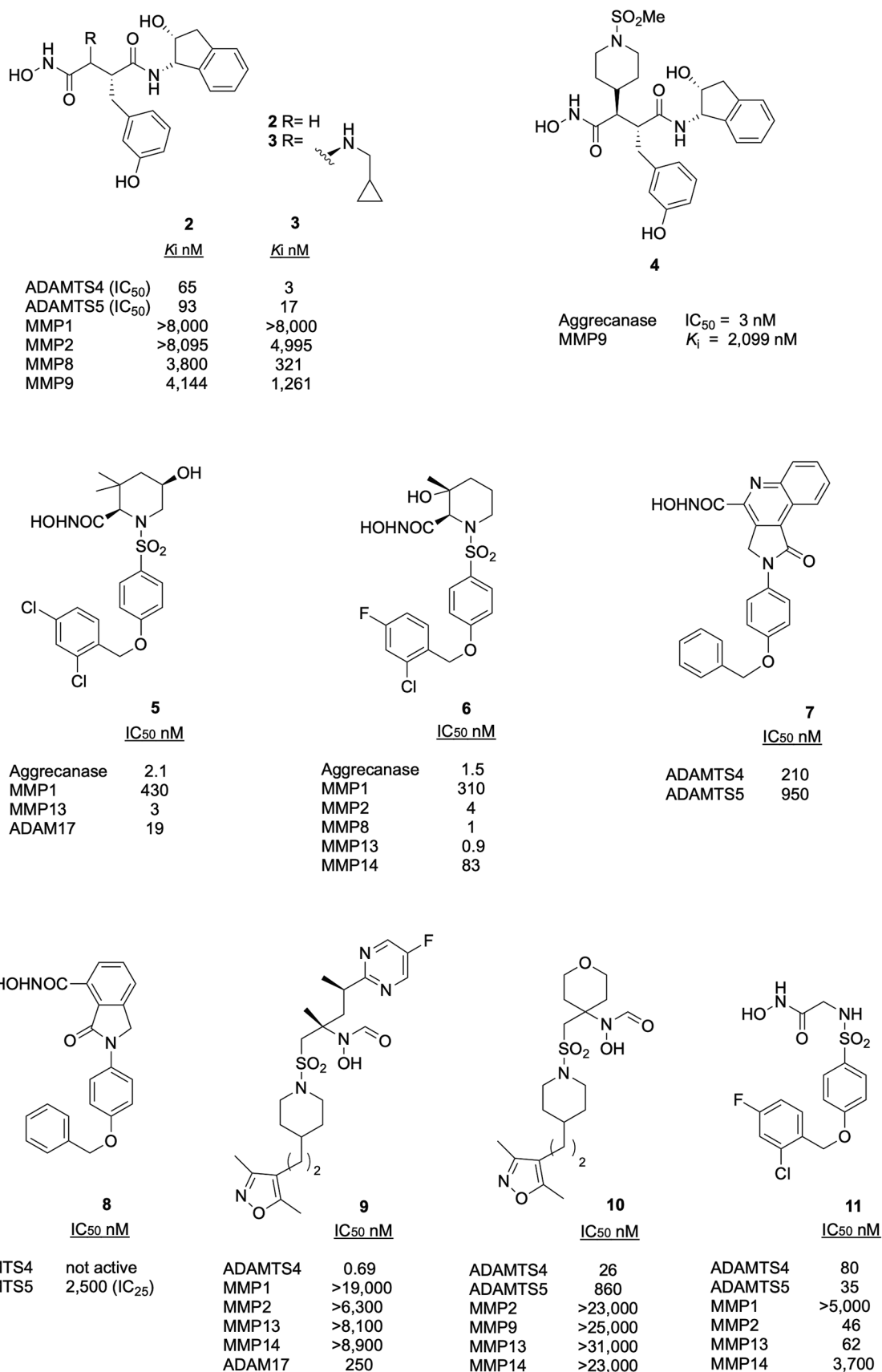
Figure 6. Inhibitory activity and selectivity profile of hydroxamate inhibitors of aggrecanases. IC 25 indicates the inhibitor concentration achieving 25% activity.
