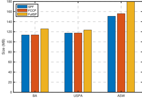
Fig. 4. Tarball sizes
