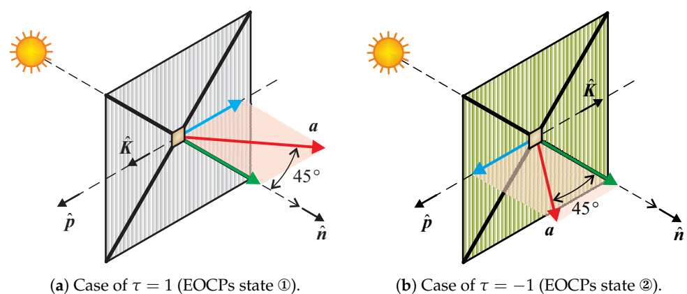
Figure 6. Propulsive acceleration components as a function of \tau and the state of EOCPs; see also Equations (2) and (3).
