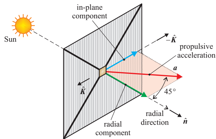
Figure 5. Propulsive acceleration vector (and its components in a body reference frame) for an ideal diffractive sail, without EOCPs, in a Sun-facing configuration.
