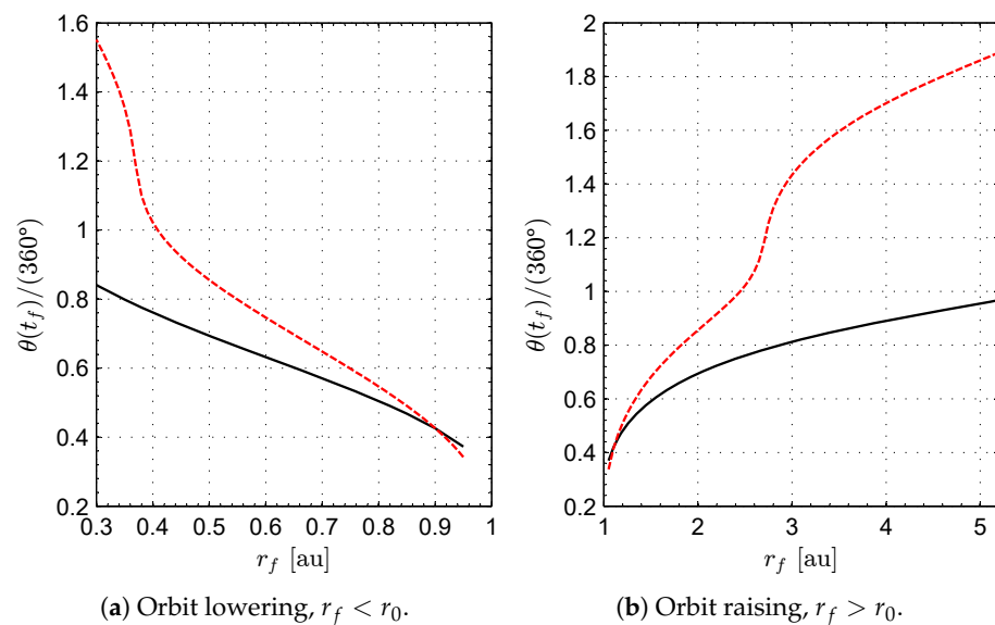
Figure 11. Final value of the polar angle as a function of the target orbit radius for an optimal transfer using an ideal and unconstrained reflective sail (red dashed line) or a Sun-facing diffractive sail with EOCPs (solid black line) when a_c = 1 \text{ mm/s}^2 .
