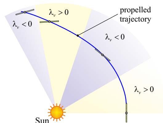
Figure 8. Sequence of trajectory arcs related to the value of the adjoint variable \lambda_v .
