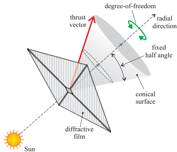
Figure 2. Single degree-of-freedom diffractive sail considered in the trajectory analysis discussed in Ref. [53].
