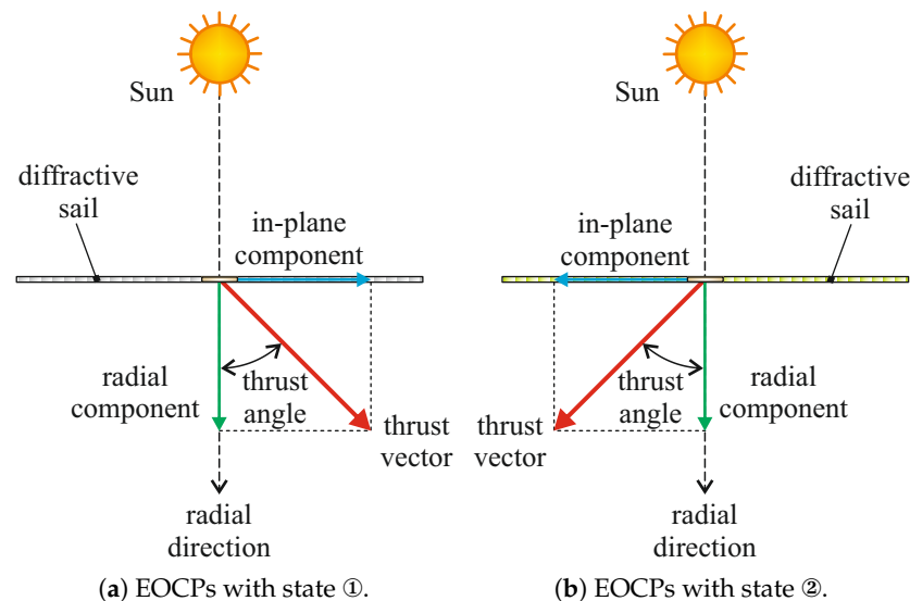
Figure 4. Diffractive sail equipped with EOCPs: conceptual sketch of the thrust vector variation as a function of EOCPs state.
