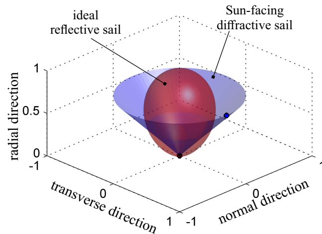
Figure 10. Force bubble of a reflective sail without attitude constraint and a diffractive sail with a Sun-facing configuration.
