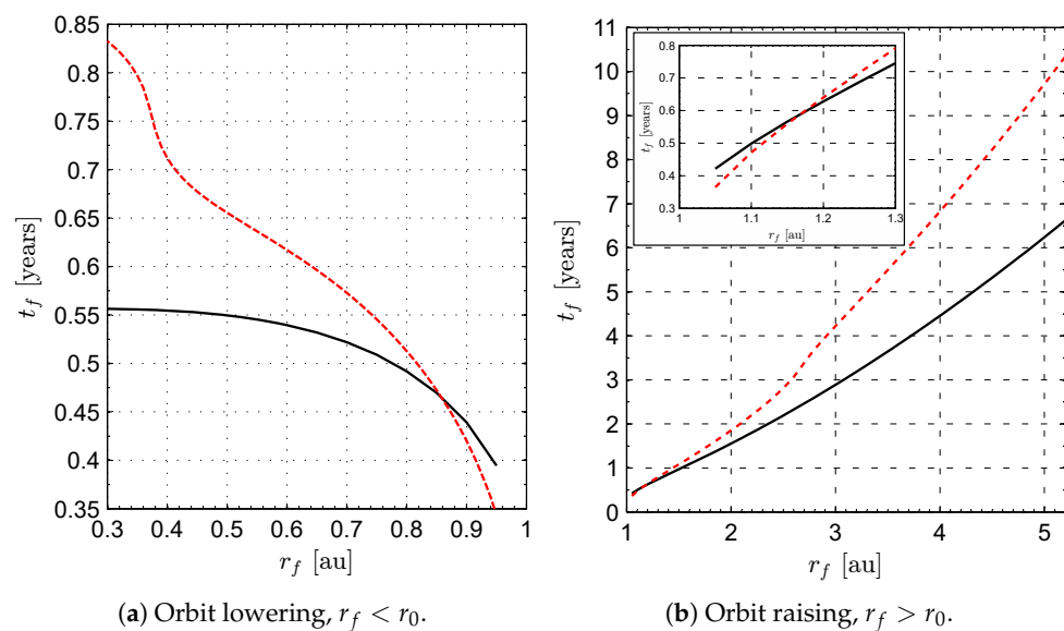
Figure 9. Minimum flight time as a function of the target orbit radius when a_c = 1 \text{ mm/s}^2 : comparison between an ideal and unconstrained reflective sail (red dashed line) and a Sun-facing diffractive sail with EOCPs (solid black line).
