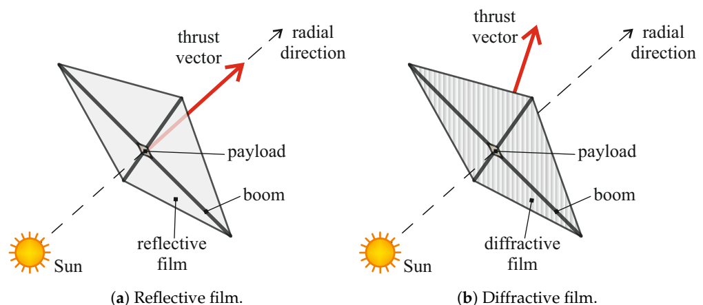
Figure 1. Conceptual scheme of the thrust vector direction in a Sun-facing solar sail with a reflective or a diffractive film.
