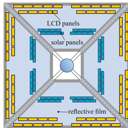
Figure 3. Conceptual scheme of JAXA's Interplanetary Kite-craft Accelerated by Radiation Of the Sun (IKAROS) spacecraft, showing active LCD panels to execute attitude control maneuvers.
