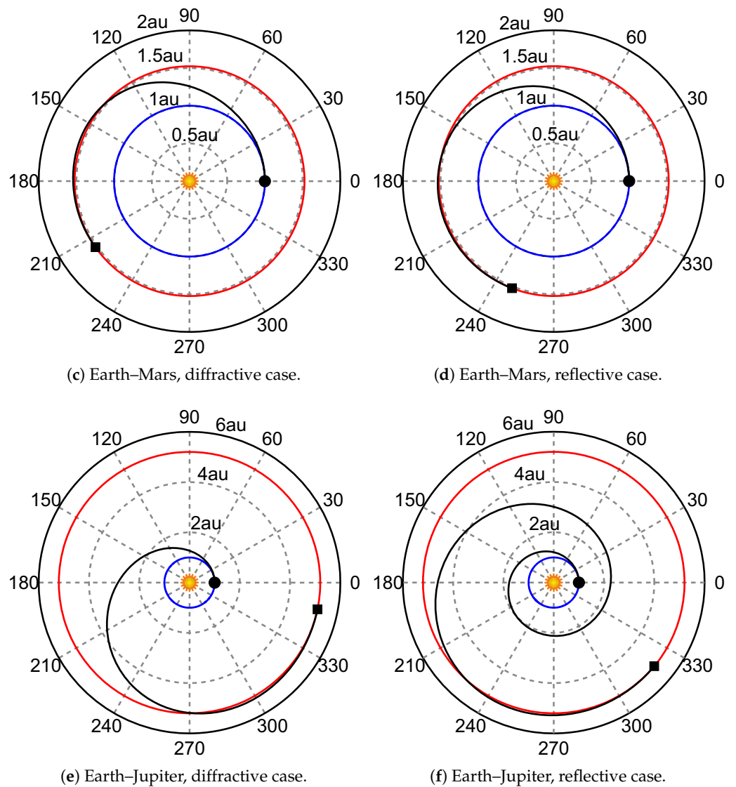
Figure 12. Optimal transfer trajectory for the three mission scenarios. Black circle → start, black square → arrival, blue line → parking orbit, red line → target orbit, black line → optimal transfer trajectory.
