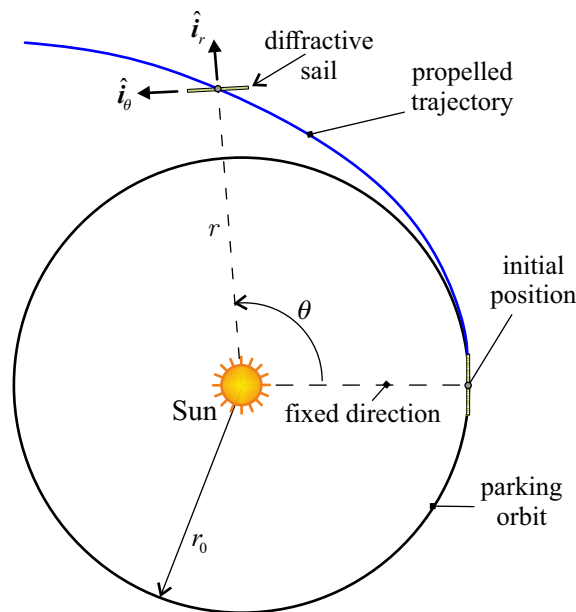
Figure 7. Polar reference frame, parking orbit, and spacecraft state variables r and \theta .
