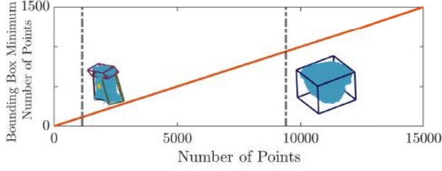
(a) \mu_b(X) = X/10 : Using a linear function, small objects are decomposed into a larger number of boxes, whereas large objects might be approximated with a single box.
