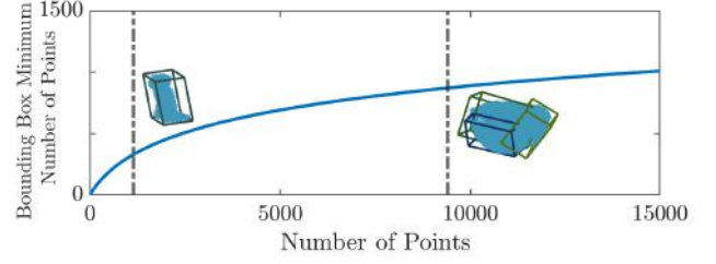
(b) \mu_b(X) = a_1 \log(a_2 X + 1) : Using a log function, small objects are decomposed into a single box, whereas large objects might be approximated by a larger number of boxes.
