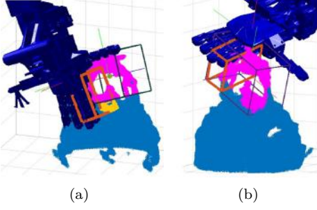
Fig. 8. Two examples of grasp poses generated for a specific box output of the box decomposition algorithm using a boiler point cloud as input. The orange box originated from the fingers of the hand is a simple model of the closing region \mathcal{C}(h) .
