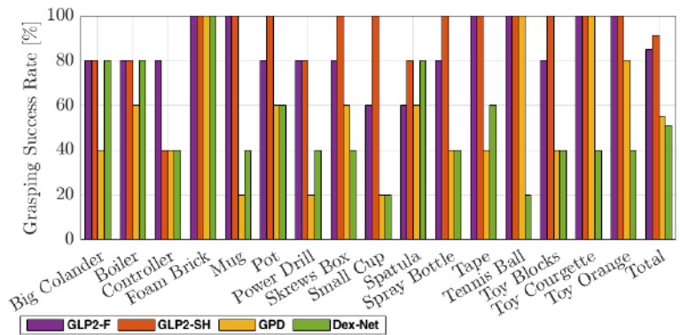
(b) Franka Hand: Grasping Success Rate (%).
