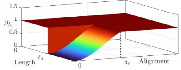
(c) Tridimensional representation of \beta_{\lambda_j} as function of the alignment and of the length.
