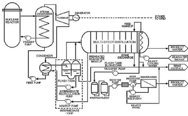
Fig. 11. Coupling between PWR and hybrid MED + RO-DP (from (Alonso, 2012)).
