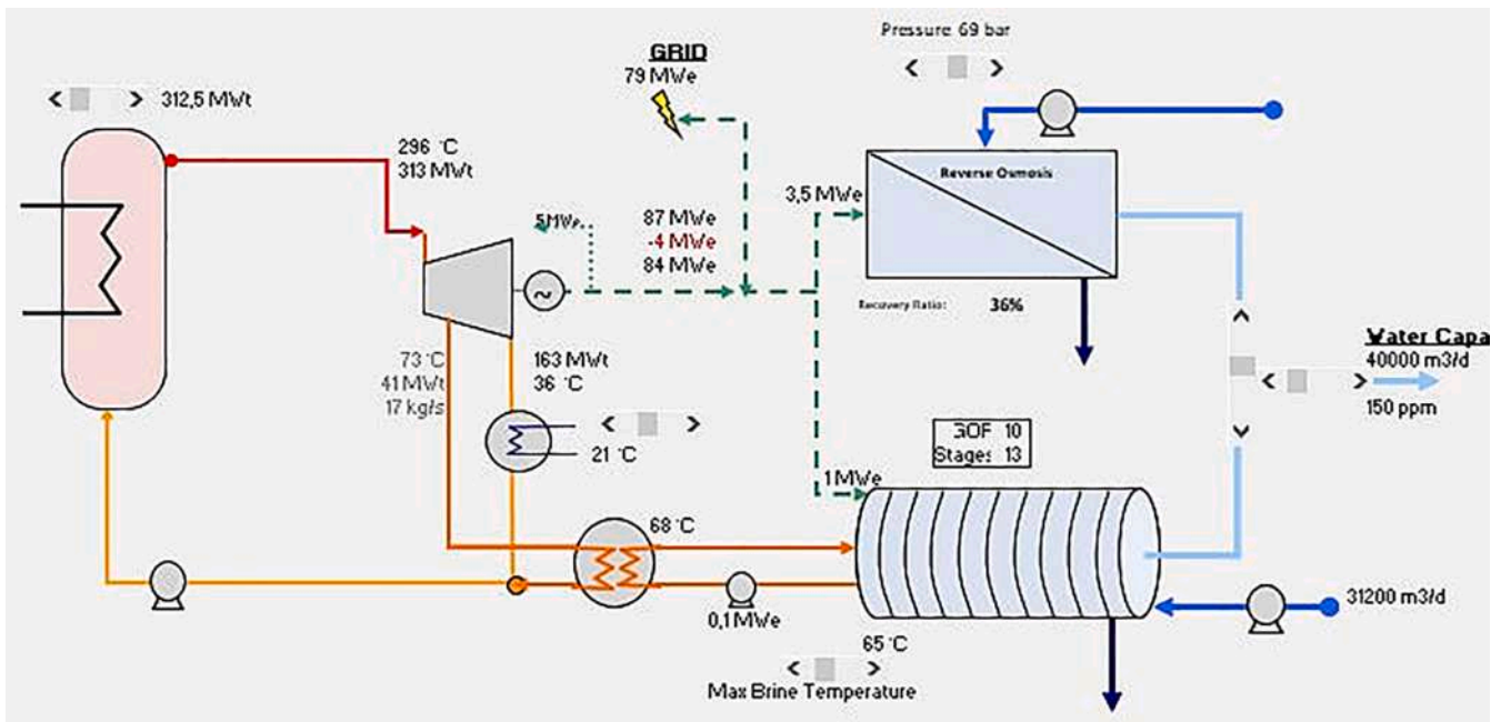
Fig. 22. Flow Diagram of SMART MED + RO (from software DEEP).
