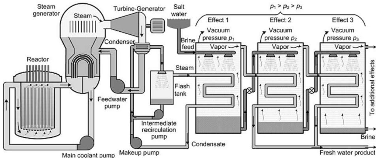
Fig. 2. Scheme of desalination plant powered with nuclear energy (courtesy from (Kazmerski and Al-Karaghoulis, 2013.1016/j.rser.2012.12.064.).
