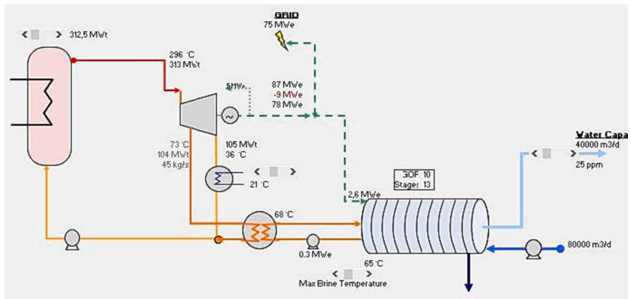
Fig. 19. Flow Diagram of SMART + MED (from software DEEP).
