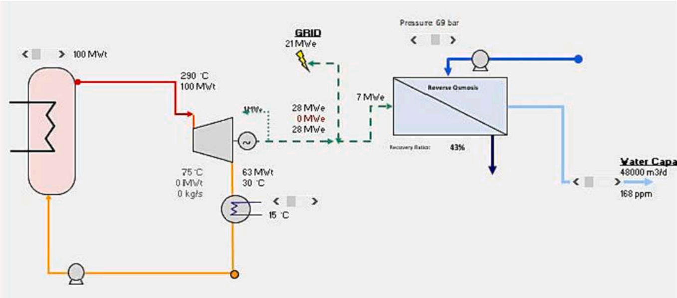
Fig. 16. Flow Diagram of CAREM + RO (from software DEEP).
