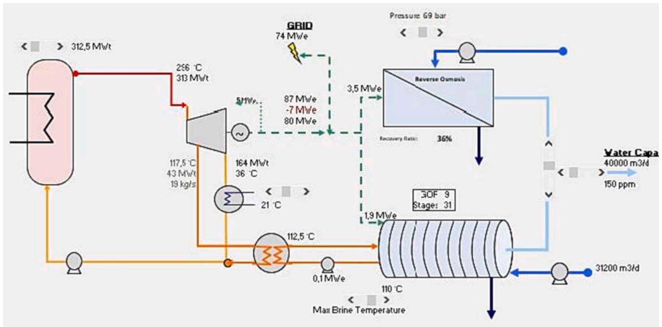
Fig. 21. Flow Diagram of SMART MSF + RO (from software DEEP).
