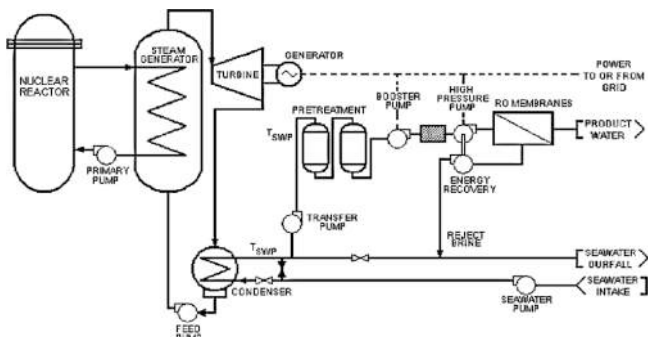
Fig. 8. Coupling between PWR and RO-DP (from (Alonso, 2012)).
