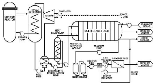
Fig. 12. Coupling between PWR and a hybrid MSF + RO-DP (from (Alonso, 2012)).
