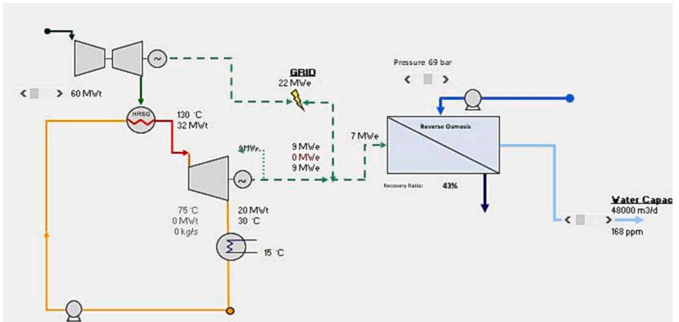
Fig. 17. Flow Diagram of CC GAS + RO (from software DEEP).
