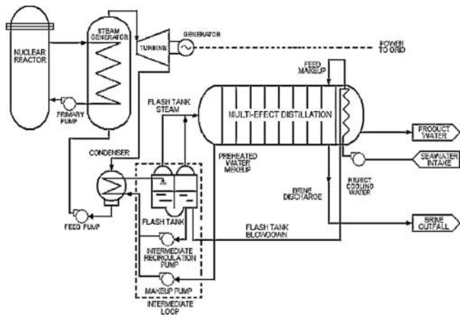
Fig. 9. Coupling between PWR and MED-DP (from (Alonso, 2012)).
