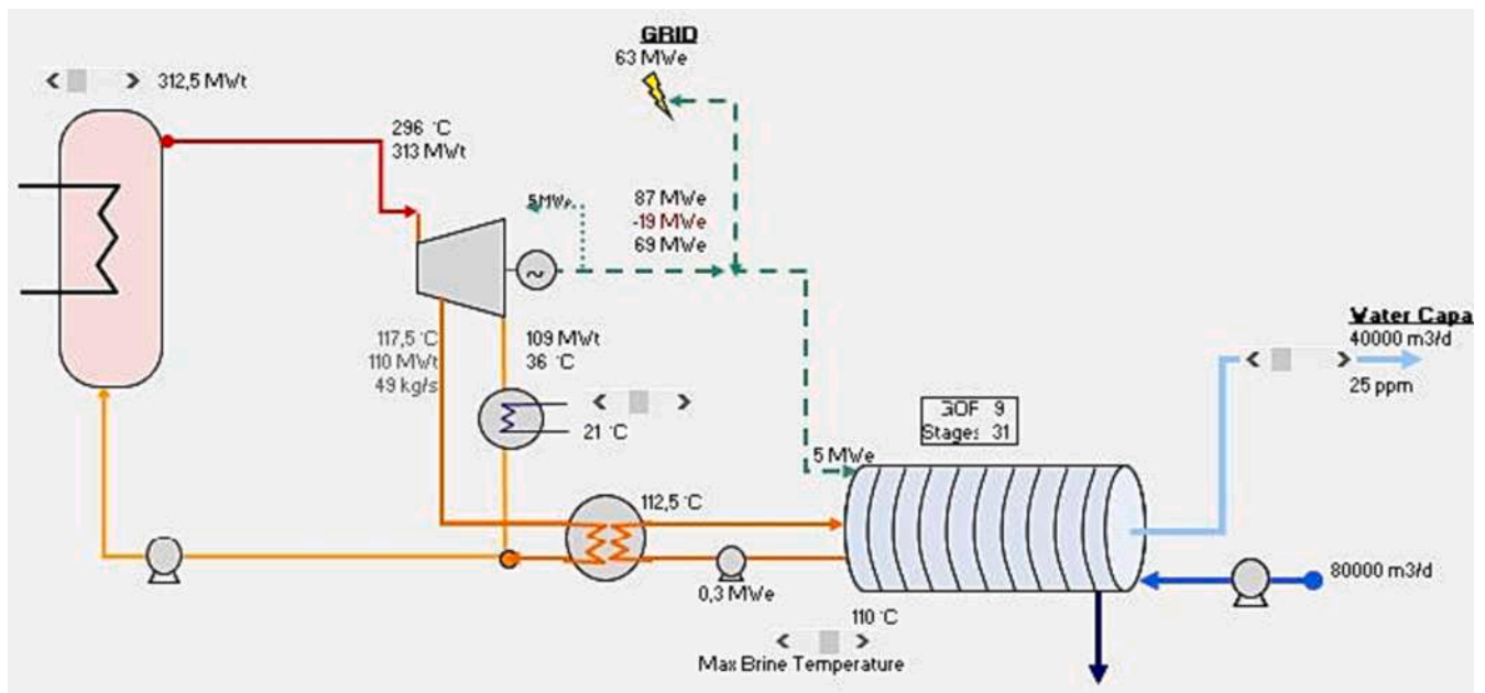
Fig. 20. Flow Diagram of SMART + MSF (from software DEEP).
