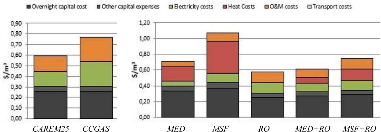
Fig. 13. Side-by-side comparison (from software DEEP).
