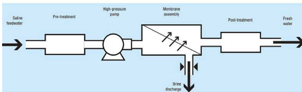
Fig. 4. RO process scheme (Schmidt and Gude, 2021).
