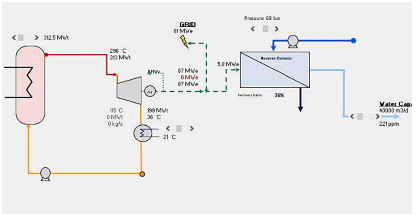
Fig. 18. Flow Diagram of SMART + RO (from software DEEP).
