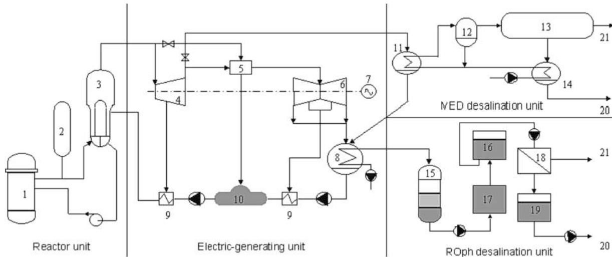
Fig. 6. Scheme of PWR-MED coupling: numbers correspond respectively to 1: Reactor core, 2: Pressuriser; 3: Steam generator; 4: High pressure turbine; 5: Intermediate steam heater; 6: Low pressure turbine; 7: Generator; 8: Main condenser; 9: Pre-heaters; 10: De-aerator; 11: Seawater heater; 12: Flash tank; 13: MED plant; 14: MED output condenser; 15: Prefilter; 16: Chlorinated water tank; 17: Ultra-filtration membrane; 18: RO membrane; 19: desalted water tank; 20: Fresh water out, 21: Brine out-fall (courtesy from (International Atomic Energy Agency, 2007)).
