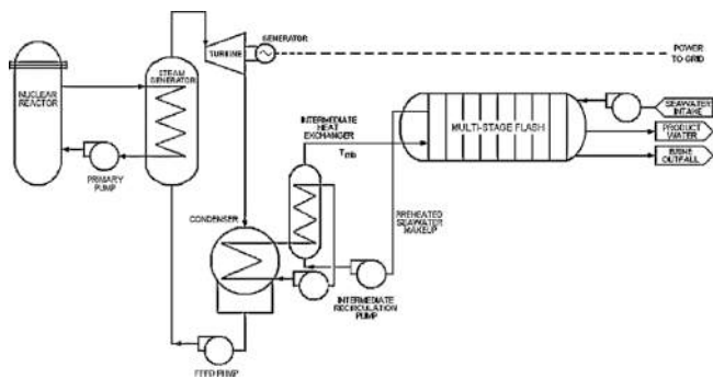
Fig. 10. Coupling between PWR and MSF-DP (from (Alonso, 2012)).
