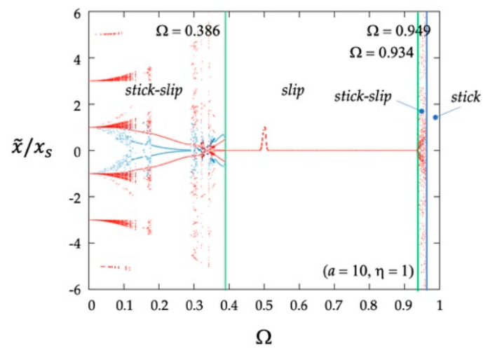
Figure 8. Bifurcation diagrams in the domain \Omega - \tilde{x}/x_s for a = 10 and \eta = 1 . Blue points on the diagram correspond to sticking phase, red points are associated with sliding phase.
