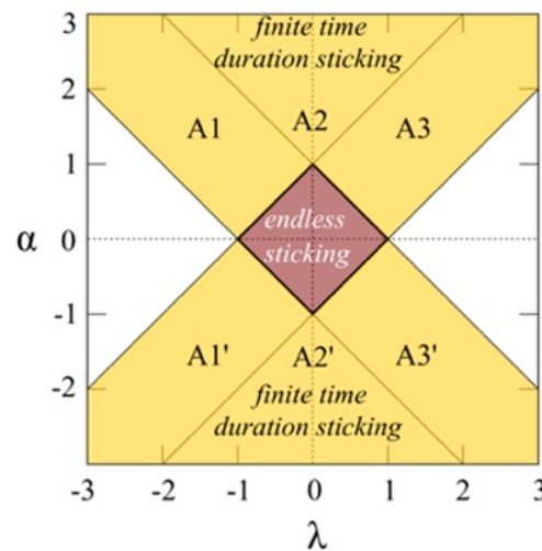
Figure 5. Sticking phase duration and corresponding reference map in the \alpha - \lambda plane.
