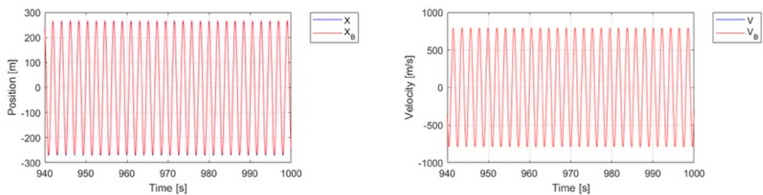
Figure 15. Time history of position and velocity for a = 10 , \eta = 1/3 , \Omega = 0.99 (sticking limit cycle).
