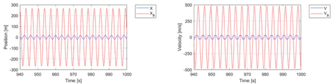
Figure 13. Time history of position and velocity for a = 10 , \eta = 1/3 , \Omega = 0.60 (sliding limit cycle).
