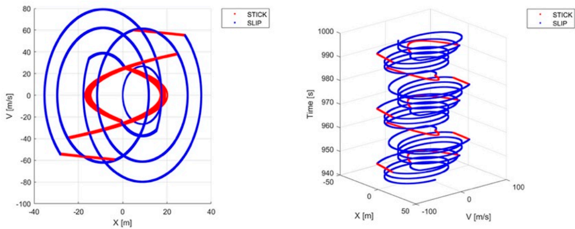
Figure 12. Phase portrait of the system for a = 10 , \eta = 1/3 , \Omega = 0.09 (stick–slip limit cycle).
