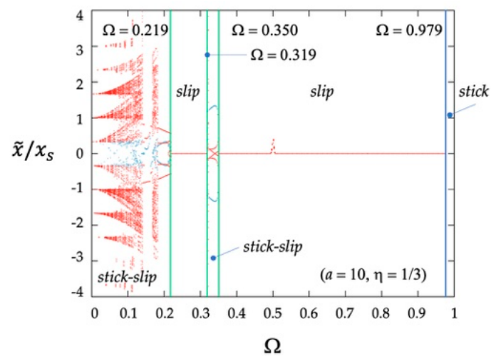
Figure 7. Bifurcation diagrams in the domain \Omega - \tilde{x}/x_s for a = 10 and \eta = 1/3 . Blue points on the diagram correspond to sticking phase, red points are associated with sliding phase.
