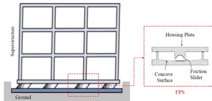
Figure 2. Example of structure fitted with a friction pendulum system (FPS adapted from [6]).
