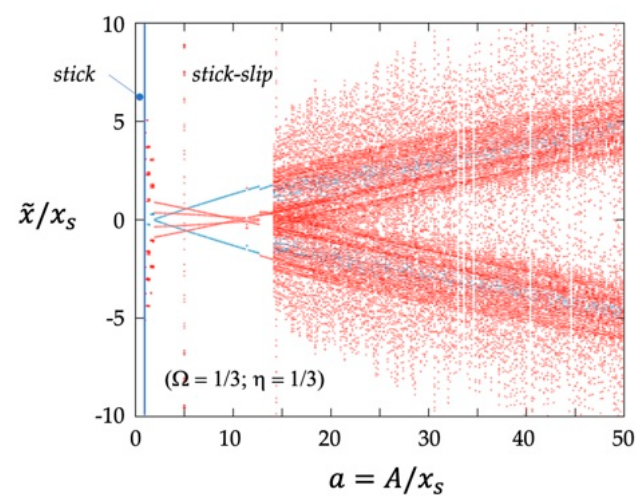
Figure 9. Bifurcation diagrams in the domain a - \tilde{x}/x_s for \Omega = 1/3 and \eta = 1/3 . Blue points on the diagram correspond to sticking phase, red points are associated with sliding phase.
