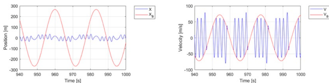
Figure 11. Time history of position and velocity for a = 10 , \eta = 1/3 , \Omega = 0.09 (stick–slip limit cycle).
