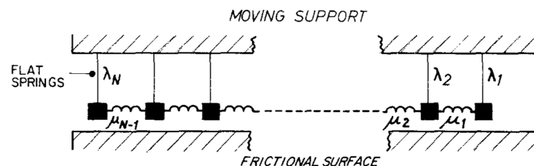
Figure 3. Schematic representation of the Burridge–Knopoff model (figure drawn from [1]).
