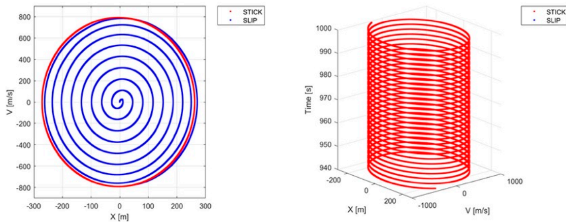
Figure 16. Phase portrait of the system for a = 10 , \eta = 1/3 , \Omega = 0.99 (sticking limit cycle).
