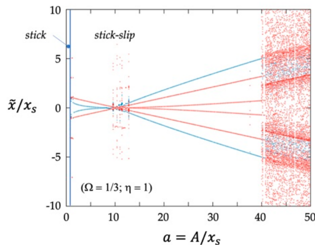
Figure 10. Bifurcation diagrams in the domain a - \tilde{x}/x_s for \Omega = 1/3 and \eta = 1 . Blue points on the diagram correspond to sticking phase, red points are associated with sliding phase.
