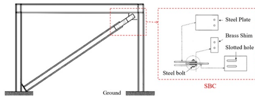
Figure 1. Example of structure fitted with a slotted bolted connection (SBC) with steel–brass sliding surfaces.
