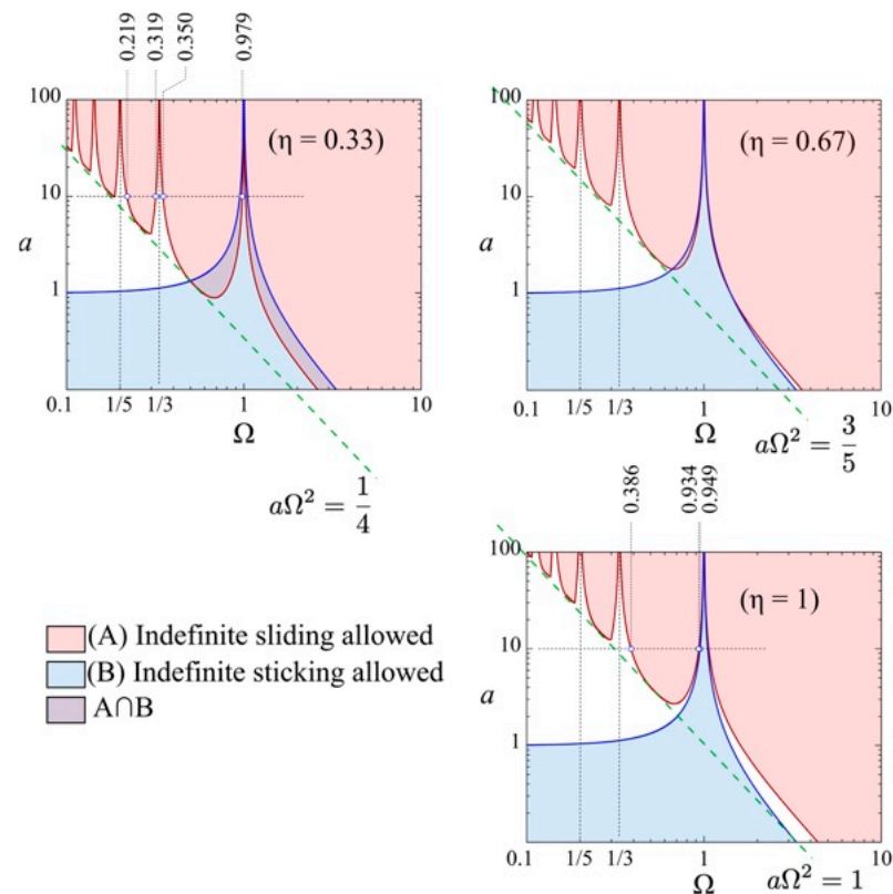
Figure 6. Partition of the a - \Omega plane showing possible long-term system responses for the three cases corresponding to \eta = 1/3 , \eta = 2/3 , and \eta = 1 .
