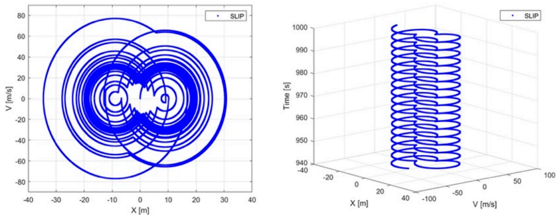
Figure 14. Phase portrait of the system for a = 10 , \eta = 1/3 , \Omega = 0.60 (sliding limit cycle).
