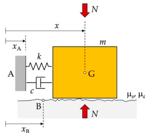
Figure 4. Scheme of a single-degree-of-freedom system that is connected elastically to a first rigid support (A) and can slide with friction over a second rigid support (B): m is the mass of the rigid block; k and c are the elastic constant of the spring and the constant coefficient of the linear dashpot between rigid block and rigid support A; \mu_s and \mu_d are the static and dynamic friction coefficients that model the tangential interaction between rigid block and rigid support B; N is the normal contact force between rigid block and rigid support B.
