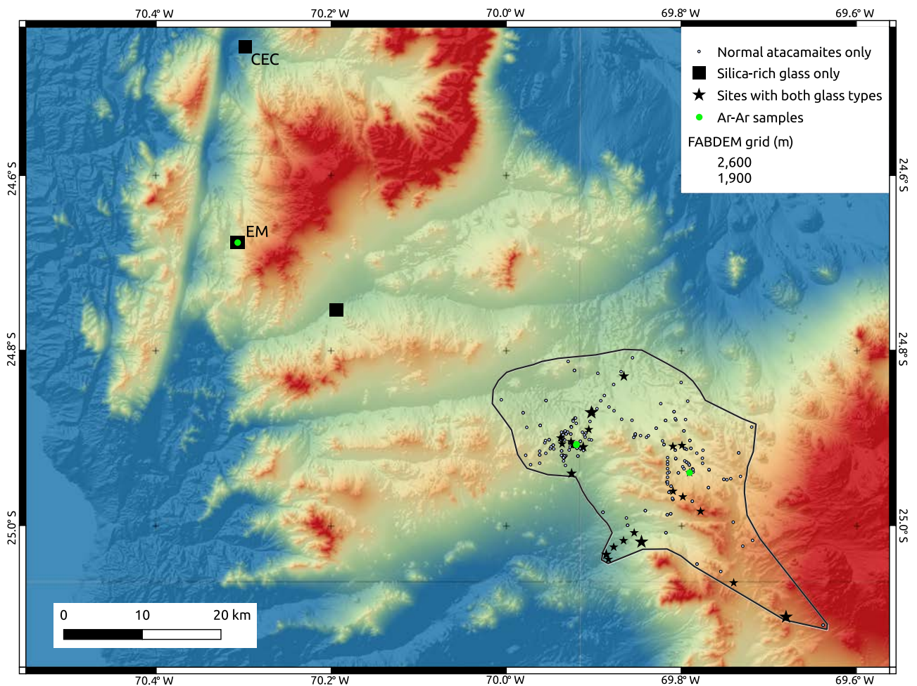
Figure 1 Map of the normal atacamite strewn field, surrounded by a solid black line, together with locations of the silica-rich glass. Large stars correspond to sites with the largest proportion of silica-rich samples.
