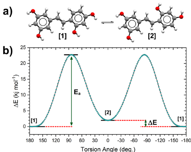
Figure 7. (a) Interconversion equilibrium between ORV forms 1 and 2. The related thermodynamic equilibrium constant is K = 0.46 . (b) The plot represents the molecular energy as a function of the dihedral angle involved in the interconversion equilibrium. \Delta E = 1.94 \text{ kJ mol}^{-1} and E_a = 22.72 \text{ kJ mol}^{-1} . The calculations were conducted by using a DFT theory level with a B3LYP functional and a 6-311+(3d, p) basis set.
