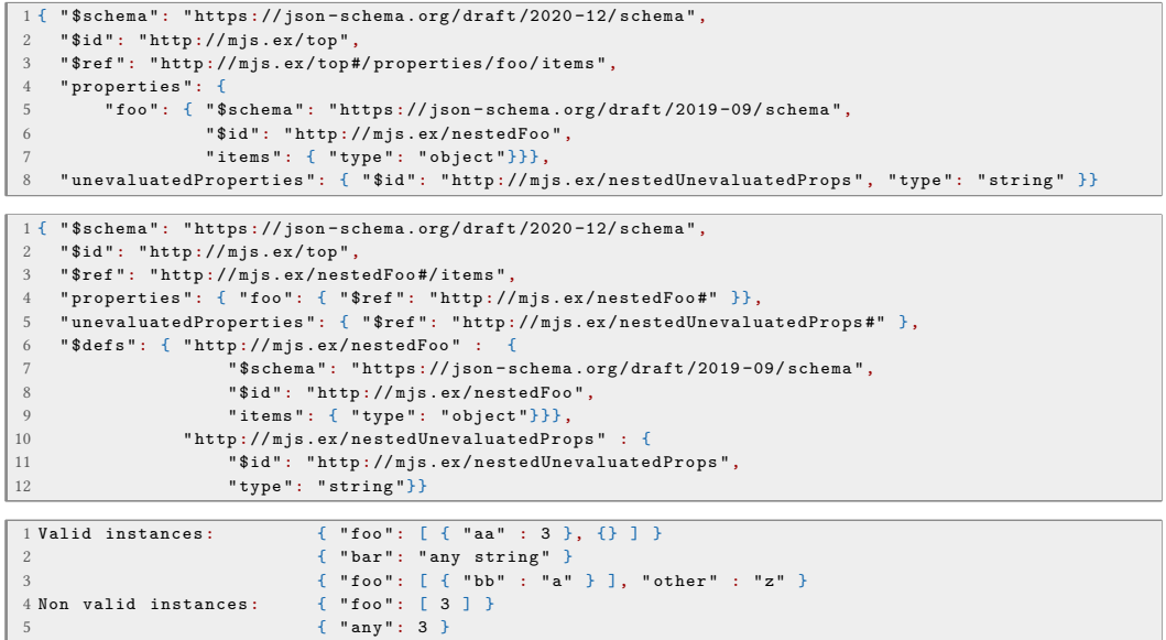
Fig. 5. A schema with embedded resources, its flattened version, and some examples.
