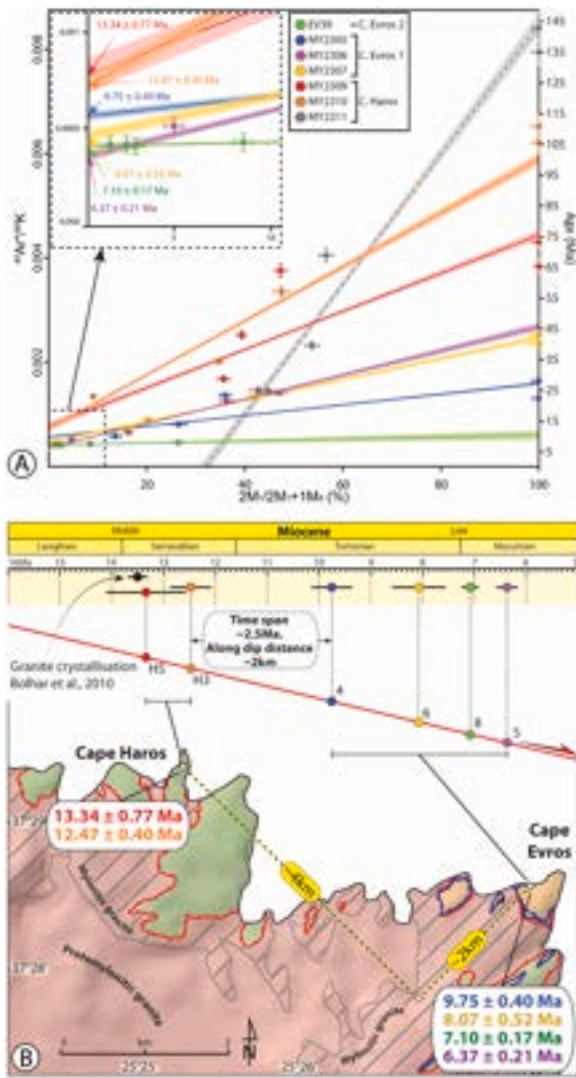
Fig. 7. (A) Illite Age Analysis by using York regression. (B) Spatial and temporal dispersion of IAA ages. The position of ages in the two outcrops is shown in panel B. See Fig. 1 for the rock unit and structural elements legend.
