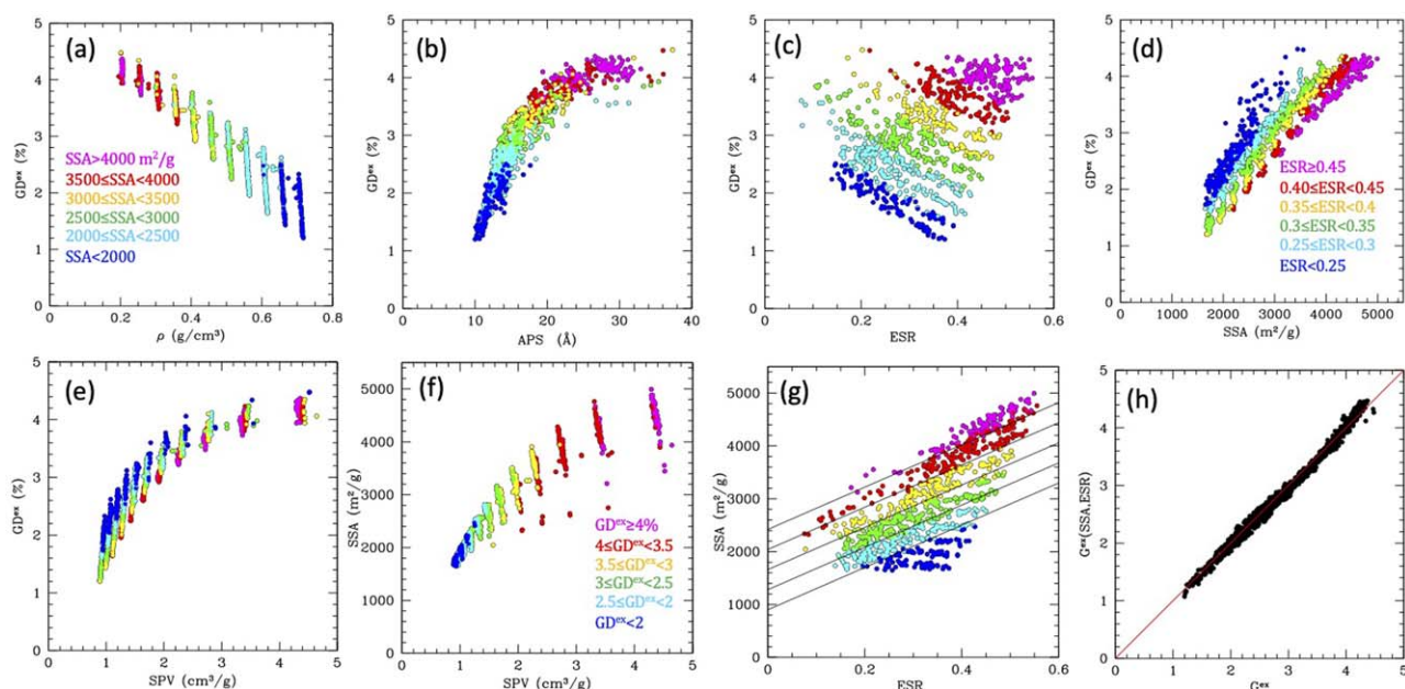
Figure 5. Dependence of H 2 adsorption on the structural parameters for the edge hydrogenated scaffolds. (a)–(c): GD ex versus density, APS and ESR, respectively, colored according to SSA (color coding reported in (a)). (d), (e) GD ex versus SSA and SPV, colored according to ESR (color coding reported in (d)). (f) and (g), SSA versus SPV and ESR, respectively, colored according to GD ex (color coding reported in (f)). The lines in (g) are eye-guides to separate the areas with increasing GD ex . Their slope is 4000 m 2 g -1 and the intercepts are evenly separated by 380 m 2 g -1 between 900 and 2420 m 2 g -1 . (h) Scatter plot between the simulated GD ex (abscissa) and the estimated G ex (ordinate) obtained with the formula GD^{ex} (\%) = 0.0013 (\text{g m}^{-2}) \text{SSA} - 5.26 \text{ESR} + 0.85 .
