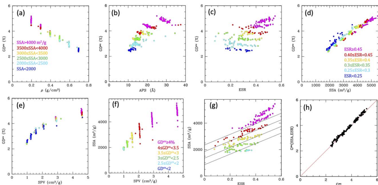
Figure 6. Same as figure 5, for non-hydrogenated-edges scaffolds. Same color coding and symbols. In (g) the lines slopes is 3000 m 2 g -1 and the intercepts are separated by 450 starting from 1200. In (h) the formula used for GD ex estimate is GD^{ex} (\%) = 0.0010 (\text{g m}^{-2}) \text{SSA} - 3.0 \text{ESR} + 1.5 .
