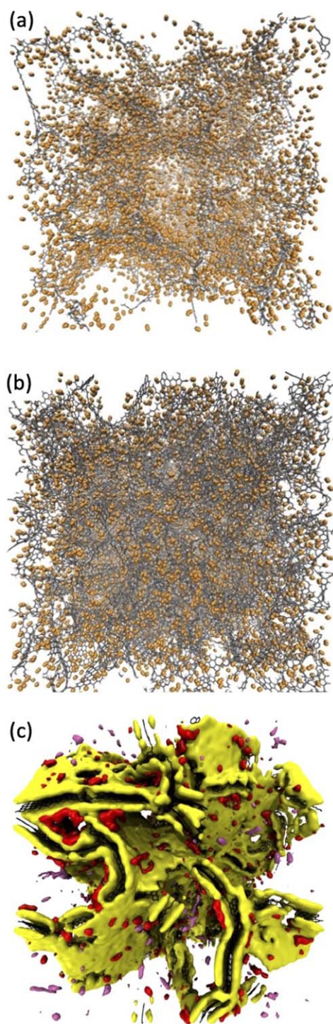
Figure 4. Scaffolds (hydrogenated-edges series) loaded with H_2 . (a) \rho = 0.2 \text{ g cm}^{-3} , ESR \sim 0.5 , ( GD \sim 4.7\% ). Scaffold atoms in grey, H_2 molecules in orange. (b) ESR \sim 0.4 , \rho = 0.7 \text{ g cm}^{-3} , ( GD \sim 2.5\% ). Same visualization as in (a). (c): \rho = 0.2 \text{ g cm}^{-3} , ESR \sim 0.25 , ( GD \sim 3.5\% ). Hydrogen molecules are represented by means of iso-density surfaces of H_2 molecules in the first layer (yellow) and in the second layer (red). Un-layered hydrogen is colored in mauve.
