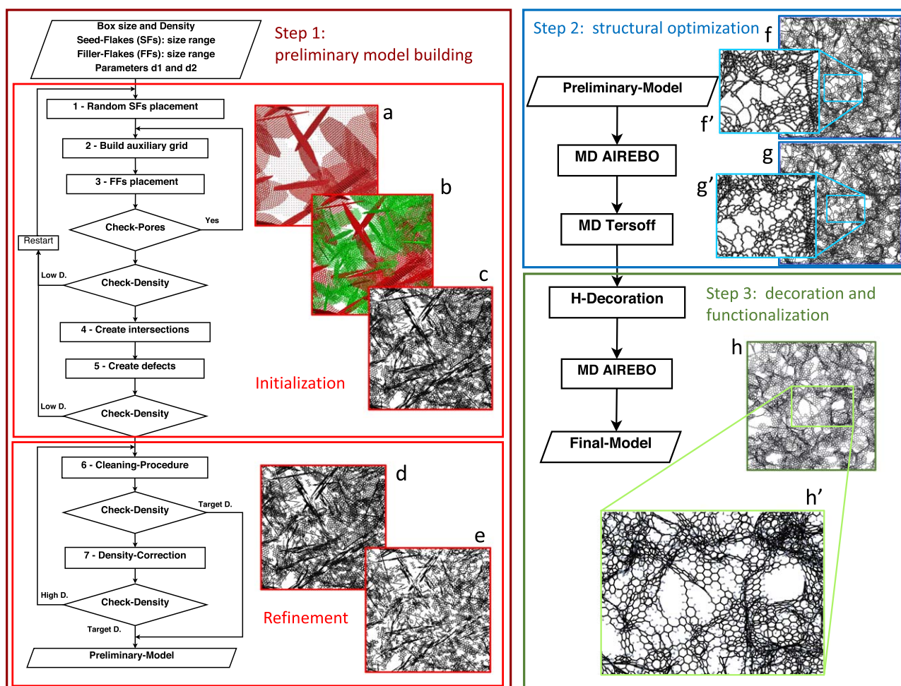
Figure 1. Scheme of the algorithm to build the models. On the left, the step 1 (red), separated in two main modules: the initialization (1–5) including the mixing of flakes (inset (a) and (b)), and their perforation (c), and the refinement (6–7, (d), (e)). Step 2 on the upper right (blue) includes the structural optimization with two different force fields: AIREBO (f, f') and Tersoff (g, g'). Step 3 (right bottom, green) includes the H-decoration of edges, and optimization with MD (h, h').
