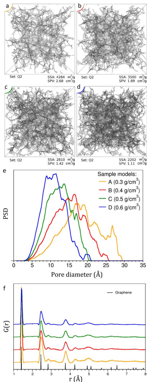
Figure 2. Sample models of hydrogenated GNMs at different densities ((a)–(d), orange, red, green and blue label, respectively; densities reported in panel (e)/(f)). The SSA and SPV values are reported within the panels. Panels (e) and (e) report the pore size distributions and the radial distribution functions in corresponding colors. The black line in panel (f) corresponds to the PDF of graphene.
