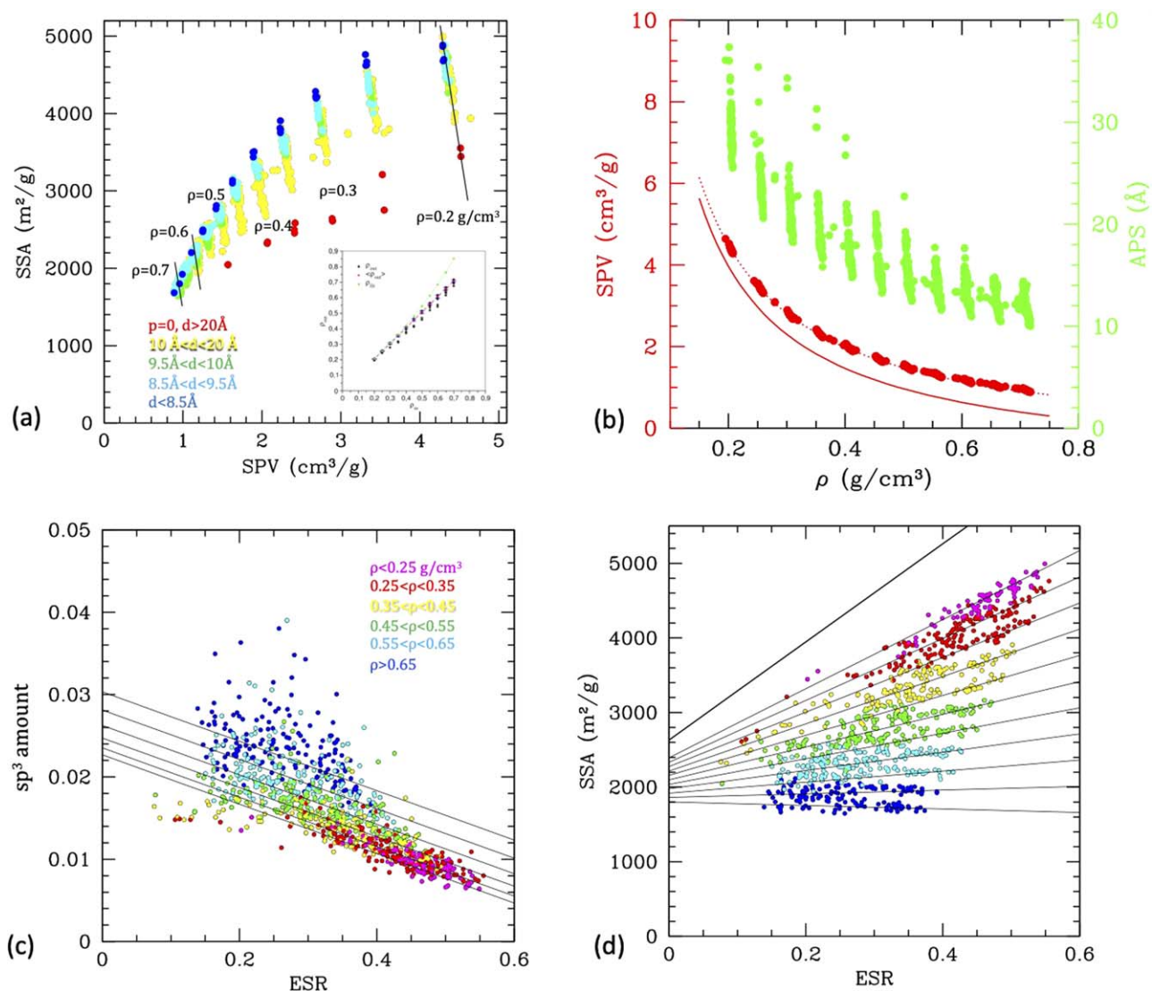
Figure 3. (a) SSA versus SPV in the whole set of generated structures. Colors from red to blue are for increasing value of the flake distance and different values of the perforation (as reported). (b) Red, unit on the left: SPV-density plot. The solid line is the analytic excluded volume formula \text{SPV} = 1/\rho - (4\pi/3)(r_C^3/m_C) , assuming all C atoms as isolated with r_C = 1.7\text{\AA} the vdW carbon radius. The dotted line is a fit, leading to r_C = 1.35\text{\AA} . Green: average pore size versus density. (c) The \text{sp}^3 amount as a function of density and of edge to surface ratio. The dots are colored according to the density as indicated in the plot. Lines are fits with the formula \text{sp}^3 = 0.017\rho^2 - 0.03\text{ ESR} + 0.022 . (d) SSA versus ESR, colored according to density (same color coding as c). The thin fitting lines are obtained with the formula in the text, with \alpha = 2.5 , A = 3.7 , B = 0.45 . The thick line is with the limit with \rho = 0 .
