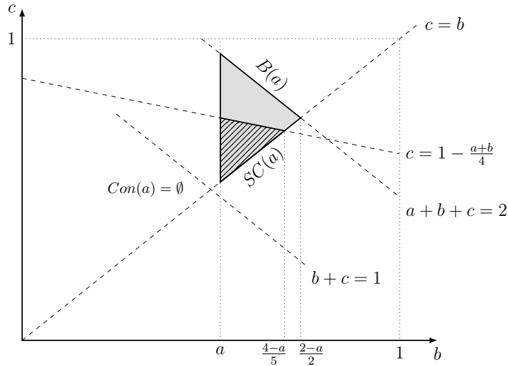
Figure 2: a > \frac{1}{2}
