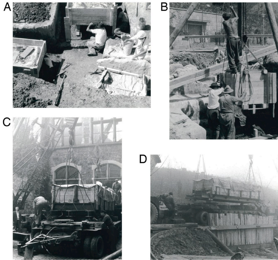
Fig. 2. A) and B) blocks lifting of the stone cist graves, C) and D) block lifting of the funerary monument by two crane trucks (Photos: Wyss 1998).
