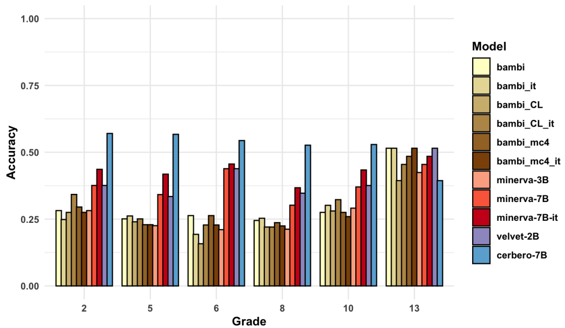
Figure 2: Accuracy reached by each model, for each grade, considering the text comprehension items.
