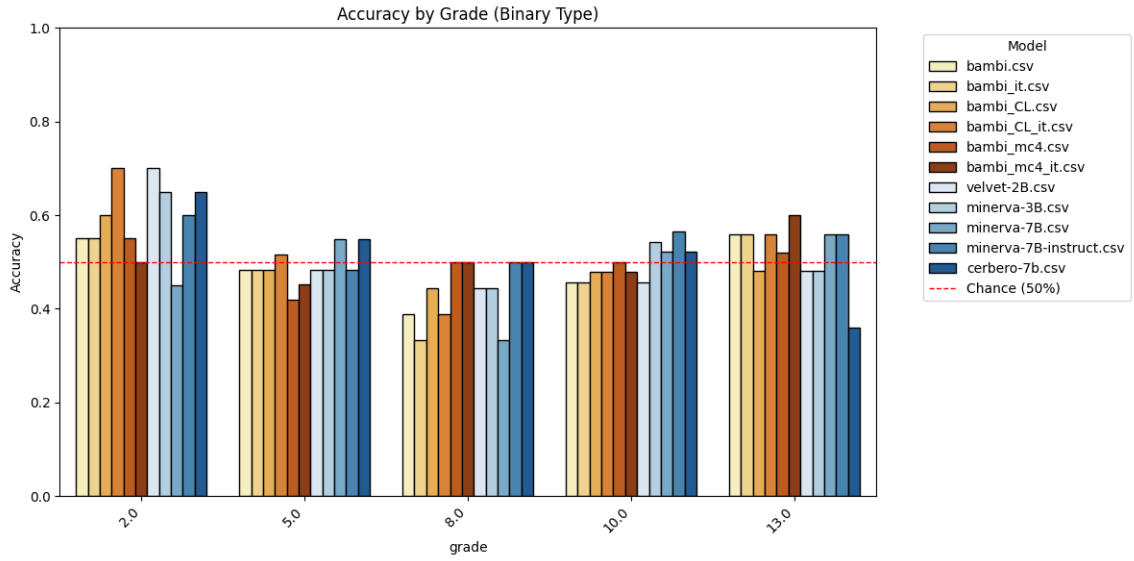
Figure 4: Accuracy achieved by all models in all grades with respect to binary questions.
