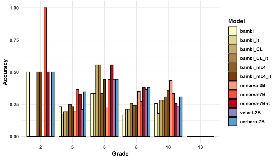
Figure 3: Accuracy reached by each model, for each grade, considering the language items.
