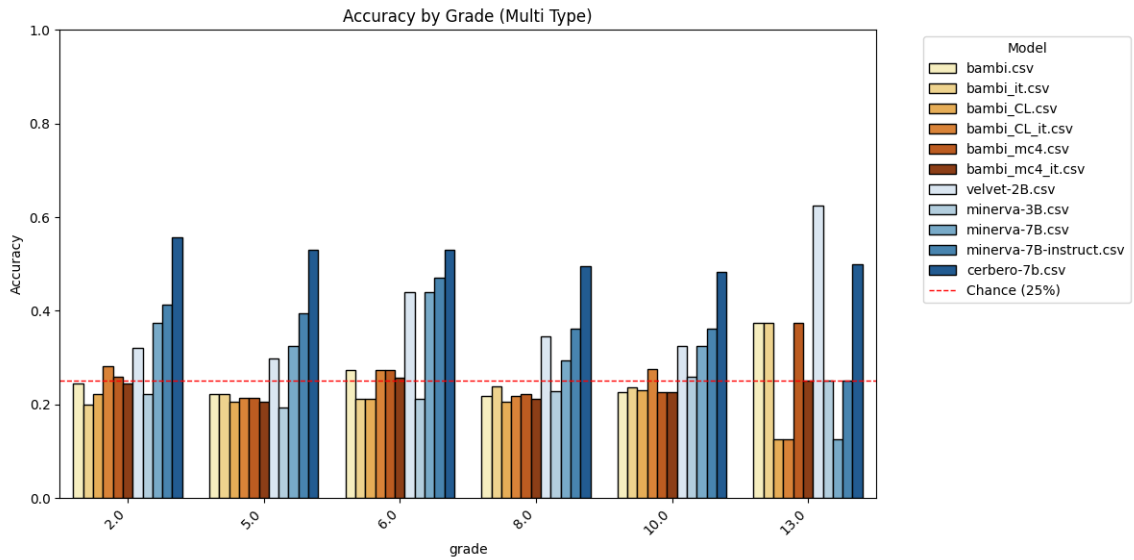
Figure 5: Accuracy achieved by all models in all grades with respect to multiple choice questions.
