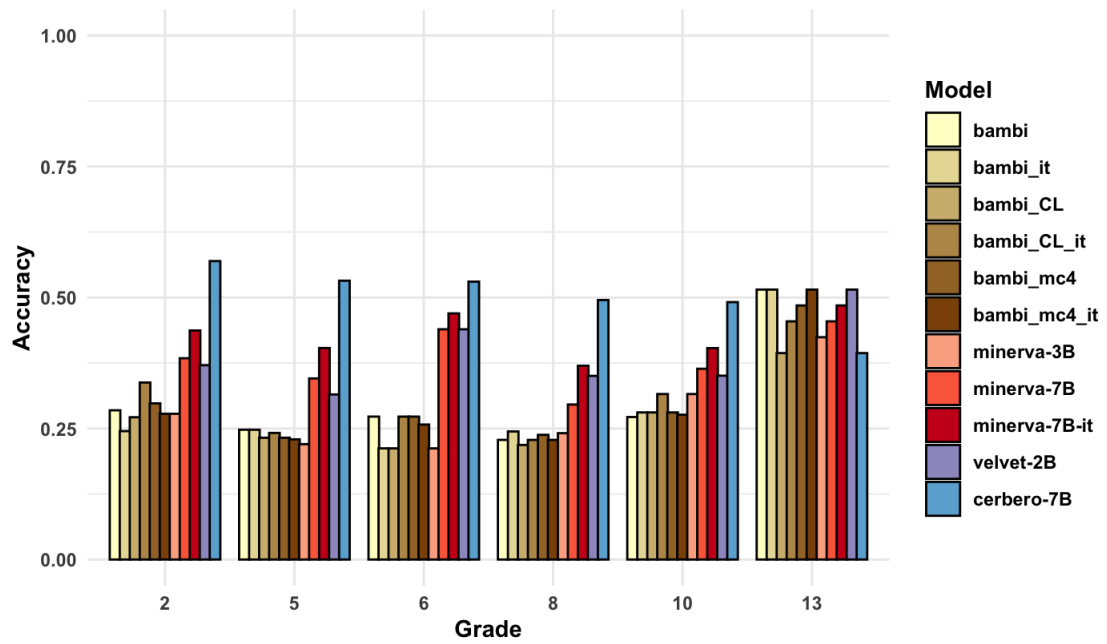
Figure 1: Accuracy reached by each model, for each grade, considering both the comprehension and the linguistic items.
