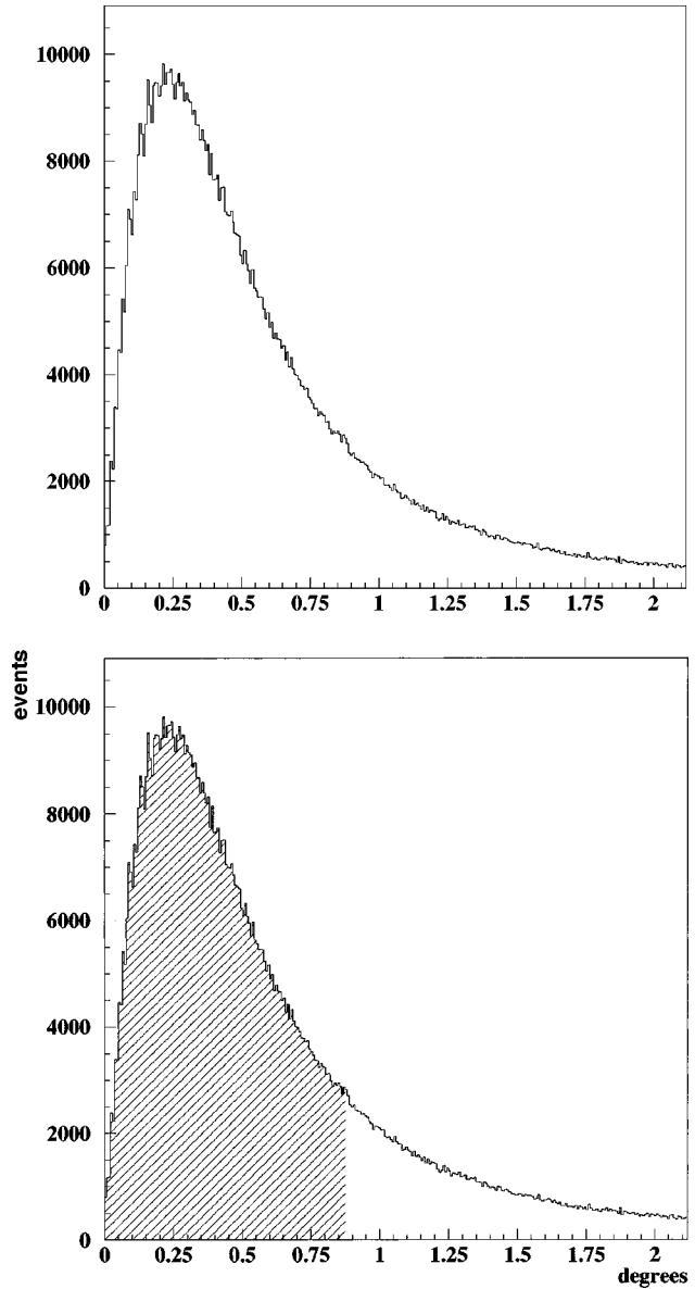
FIG. 8. The space angle distribution of double muons. The angular resolution of the MACRO apparatus, defined as the cone angle containing 68% of the events from a point source, is shown as a shaded region. With this definition, MACRO's angular resolution is 0.90^\circ .
