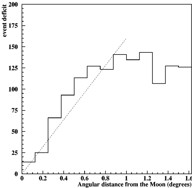
FIG. 2. Integral event deficit vs angular distance from the Moon center. Superposed on the integral event deficit is an approximate fit to the distribution out to 0.9^\circ : \Delta N^{def} = 165\alpha , where \alpha is the angular distance from the Moon center.
