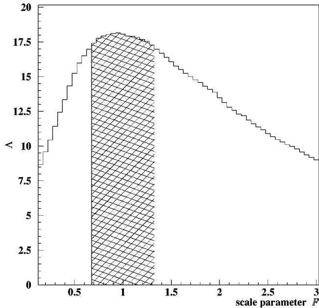
FIG. 7. The distribution of \Lambda as a function of \mathcal{F} . The maximum \Lambda , \Lambda^* , is found for \mathcal{F}=1.0 . The shaded area shows the region where \Lambda^* falls by 1.0, or the 1\sigma confidence interval for \mathcal{F} [3].
