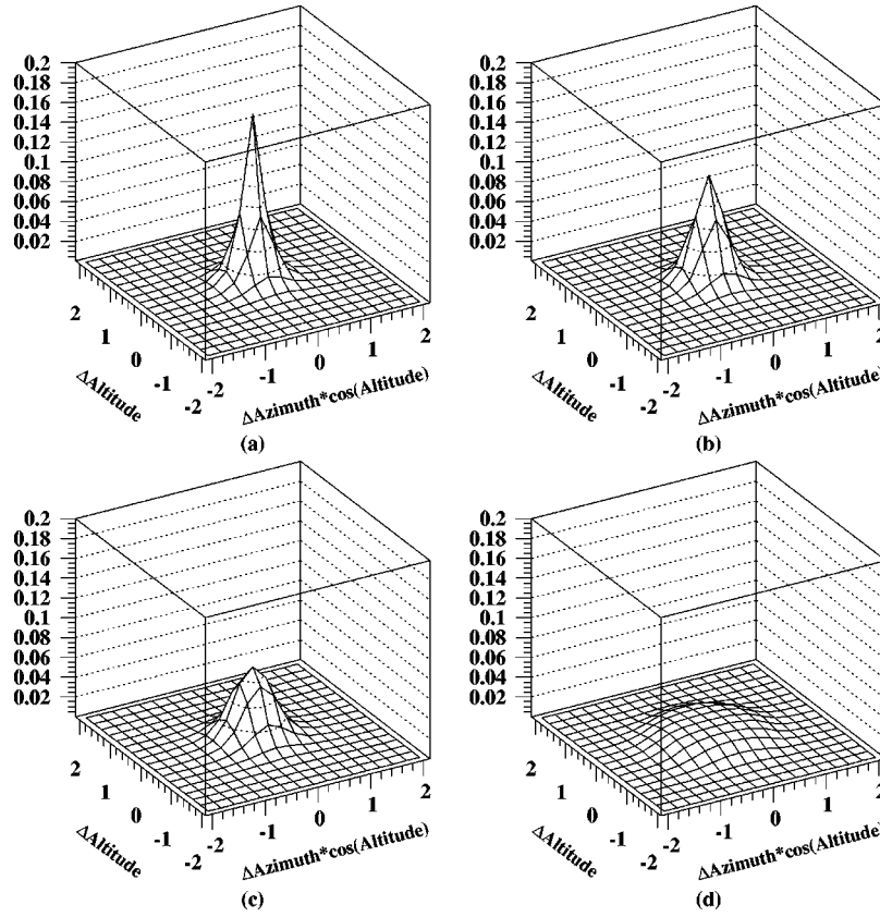
FIG. 4. (a) The MPSF, normalized to unit area from Fig. 3(a). (b) The MPSF modified by a disk of radius 0.26^\circ , the average lunar radius, and then normalized to unit area; this is the modified MPSF used in the likelihood analysis. (c) The MPSF modified by a disk of radius 0.4^\circ and then normalized. (d) The MPSF modified by a disk of radius 1.0^\circ and then normalized.
