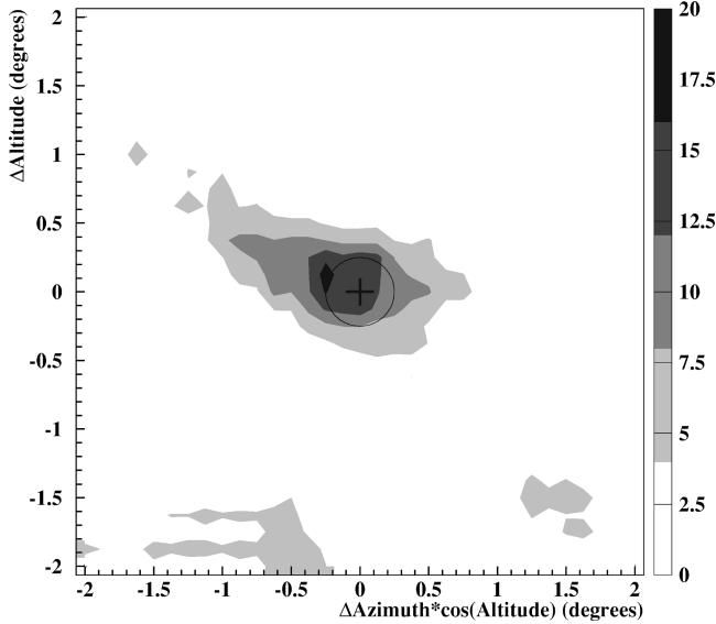
FIG. 5. The two dimensional distribution of \lambda in bins of equal solid angle in the Moon window. The axes are offsets from the Moon center. The fiducial position of the Moon, at position (0,0) , is marked by a + ; a circle corresponding to the average lunar radius, 0.26^\circ , is centered at this position. The \lambda grey scale is given at the right margin of the figure. The maximum of this distribution, \Lambda=18.3 , is offset from the fiducial Moon position at \Delta azimuth =-0.25^\circ and \Delta altitude =+0.125^\circ .
