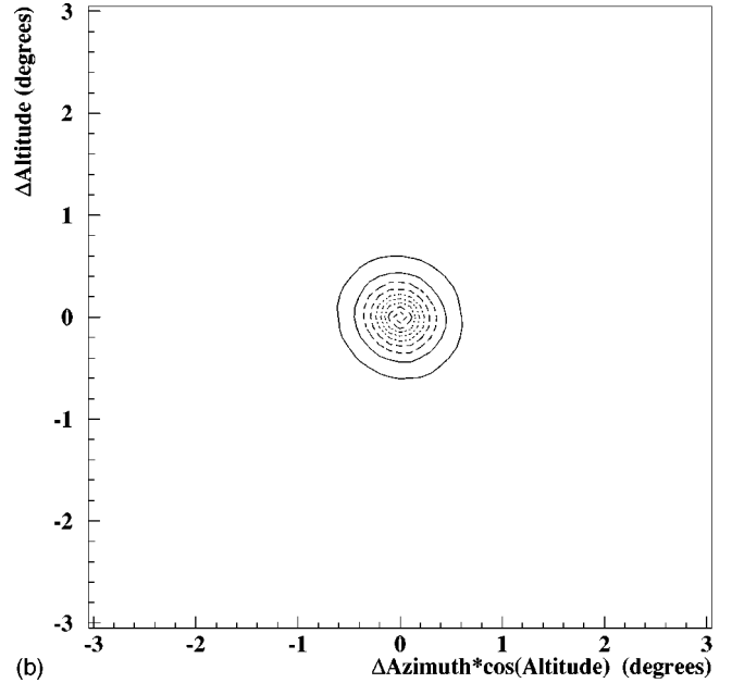
FIG. 3. (a) The point spread function of the MACRO apparatus (MPSF) derived from the space angle distribution of 1 044 877 double muons. (b) Contour diagram of the MPSF. The contours levels are equally spaced between 2000 and 18 000 muons. The MPSF is circularly symmetric in this coordinate system.
