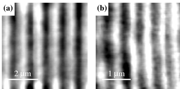
FIG. 1. Birefringence NSOM images ( \lambda = 690 nm) of optical gratings realized by previously tracing parallel vertical lines with the NSOM probe ( \lambda = 488 nm) on a thin film of PMA4. The lines are spaced by (a) 1000 nm, and (b) 500 nm.
