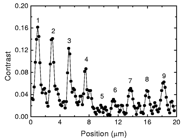
FIG. 2. Processed line profile obtained from birefringence NSOM images of nine vertical lines ( 2\text{-}\mu\text{m} spaced) imprinted with different scan speeds: from left to right, four lines at 300 \text{ nm/s} , one line at 10 \mu\text{m/s} , and four lines at 3 \mu\text{m/s} .
