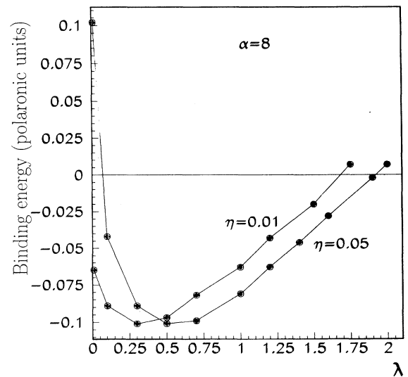
FIG. 2. Binding energies of the bi-plasma-polaron are shown as function of \lambda for \alpha = 8 and \eta = 0.01 and 0.05. \lambda = 1 indicates an electronic density of 4.45 \times 10^{19} \text{ cm}^{-3} . The energies are in units of \hbar\omega_l .
