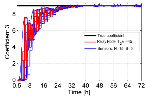
Fig. 14. Example of a non-zero coefficient estimate versus time. The sensors and the RN gradually reach the consensus after about 48 hours.
