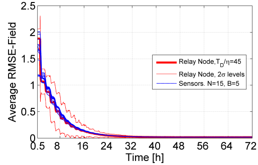
Fig. 12. Field RMSE (averaged over 100 Monte Carlo runs) versus time of the RN and the sensors for \gamma = 45 .
