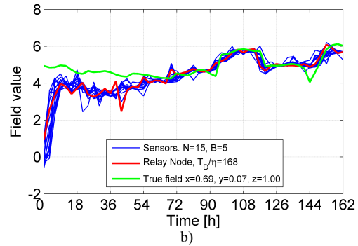
Fig. 22. Sensors and RN estimated field at a given position sub-sampled every 3 hours. a) The transition phase duration of the field estimates is about 18h after that the estimates track the true NCOM field variations. b) The transition phase duration in this second case is about 72h after that the estimates start to track the true NCOM field variations more closely.
