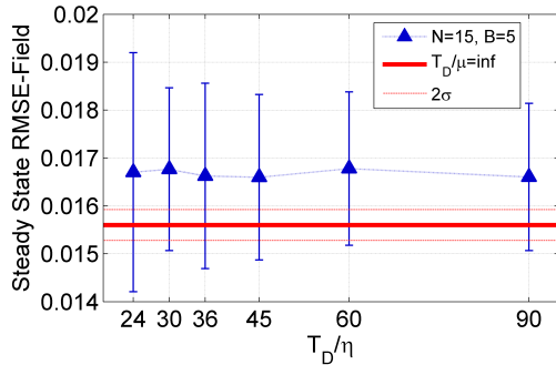
Fig. 10. Steady state field RMSE at the RN as function of \gamma = T_D / \eta compared with the centralized consensus solution. Constant coefficient case.
