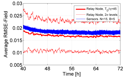
Fig. 13. Field RMSE (averaged over 100 Monte Carlo runs) versus time of the RN and the sensors for \gamma = 45 . Zoom in of the steady state phase.
