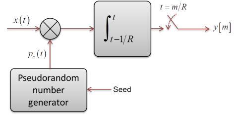
Fig. 2. Random demodulator scheme. Adapted from Tropp et al [17].
