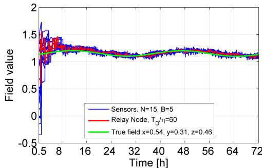
Fig. 16. Estimated field from sensors and fusion center at given position.
