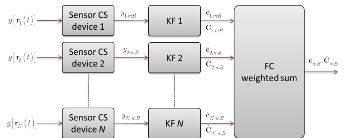
Fig. 3. Centralized Kalman filter estimation from CS samples of the scalar field.
