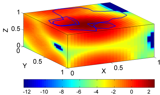
Fig. 11. Estimated field (natural logarithmic scale) at the end of the observation period with optimal trajectory for sensor 15 projected on the horizontal plane.
