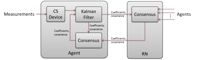
Fig. 6. Agent and RN structure.
