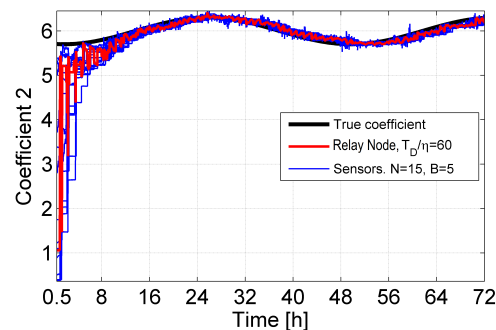
Fig. 19. Example of non-zero coefficient for the sinusoidal case. The sensors and the fusion center gradually reach a consensus after 16 hours and track the coefficient variations.
