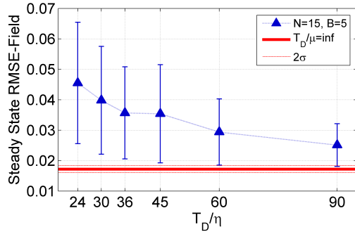
Fig. 15. Steady state field RMSE at the RN as function of \gamma = T_D / \eta compared with the centralized consensus solution. Sinusoidal coefficient case.
