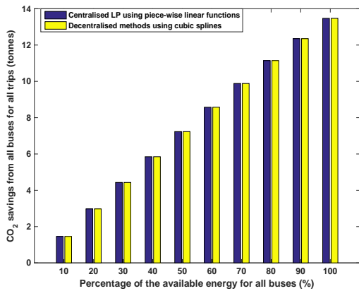
Fig. 10: Overall CO_2 savings of all PHEBs with respect to different percentage of energy available.
