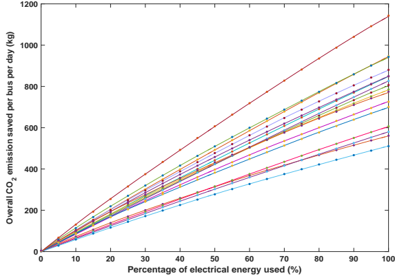
Fig. 3: Utility functions of 16 PHEBs in Dublin city (considered outside the greenzone). Note that some buses pollute more than others (and thus, have a greater potential in terms of CO_2 savings) depending on the characteristics of their routes (e.g., speed limits, traffic conditions, topography of the route). The “.” points are fitted using cubic splines. For the trips passing by the city centre, we here show the utility functions corresponding to the part of the trip outside the green zone (for which the driving mode has to be decided).
