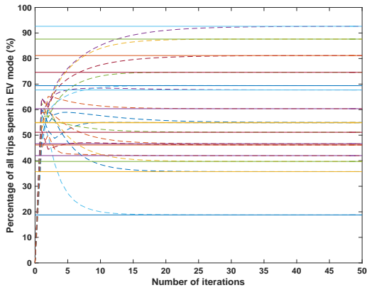
Fig. 9: Evolution of the distributed ADMM.
