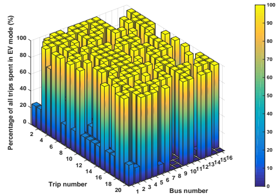
Fig. 6: Percentage of electric energy used for all PHEBs of all their trips.
