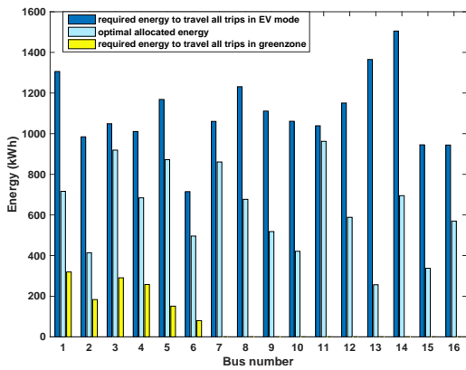
Fig. 4: Comparison of different energy consumption patterns for 16 PHEBs.
