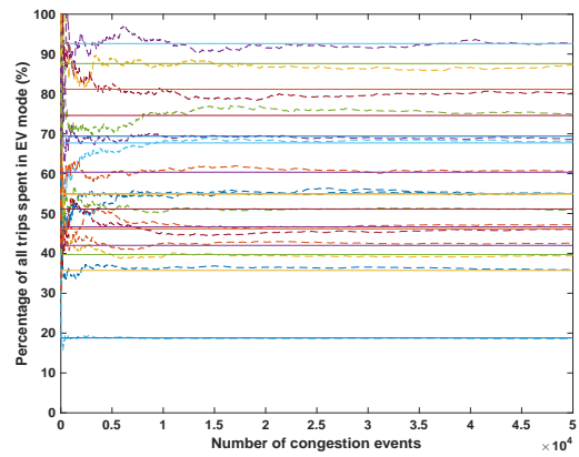
Fig. 7: AIMD converges to the correct solution.
