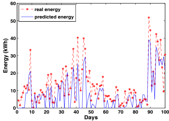
Fig. 12: Comparison between the real and the predicted energy generated from PV panels in UCD.
