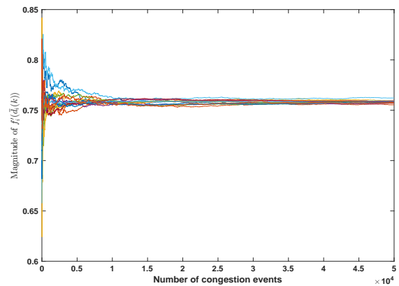
Fig. 8: The derivatives of the utility functions converge in a consensus fashion.
