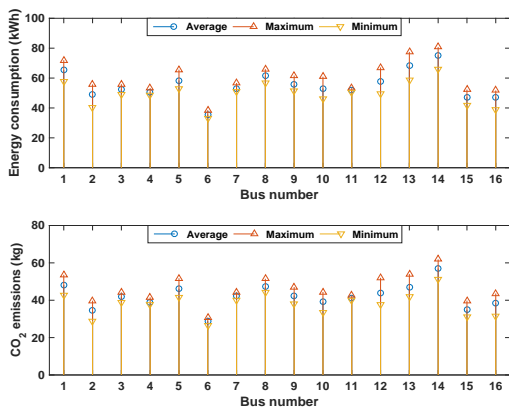
Fig. 5: Energy consumption and emission generation patterns for all bus routes.
