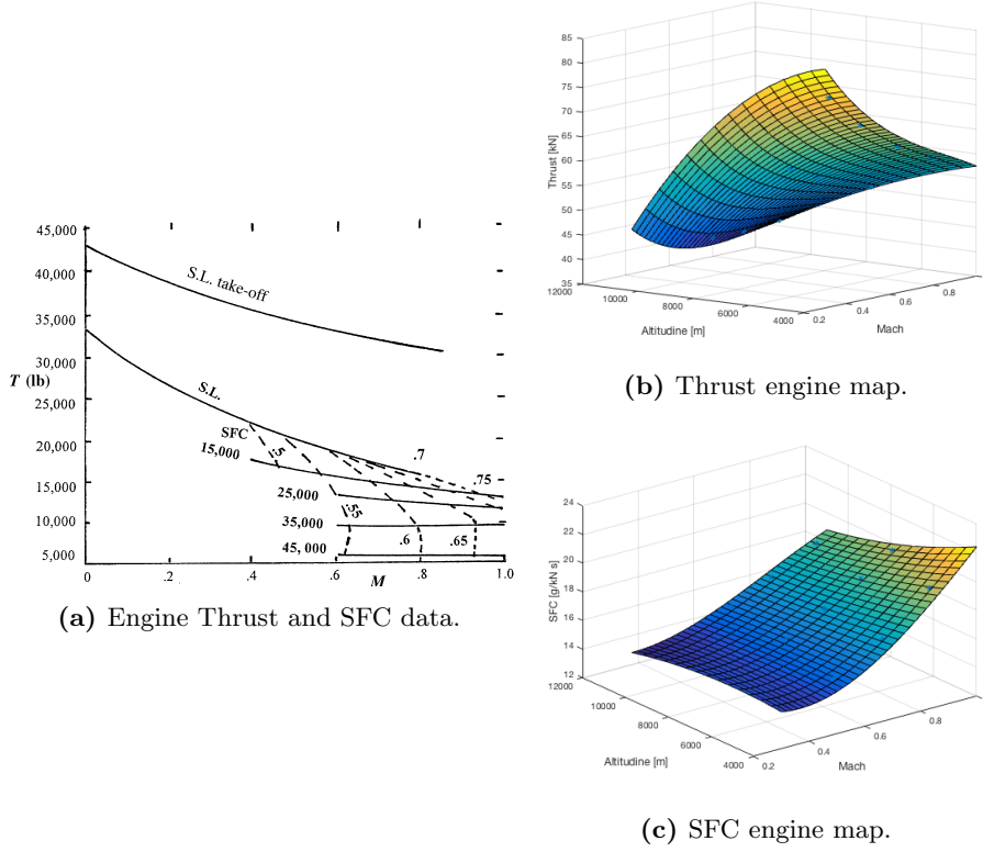
Fig. 6: Engine characteristics.
