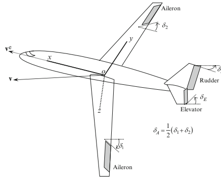
Fig. 5: Surface controls of the aircraft, from [22].
