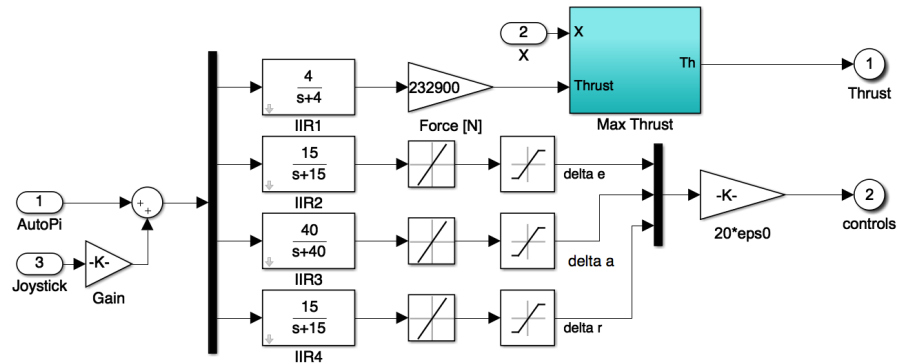
Fig. 10: Actuators dynamics and engine model.
