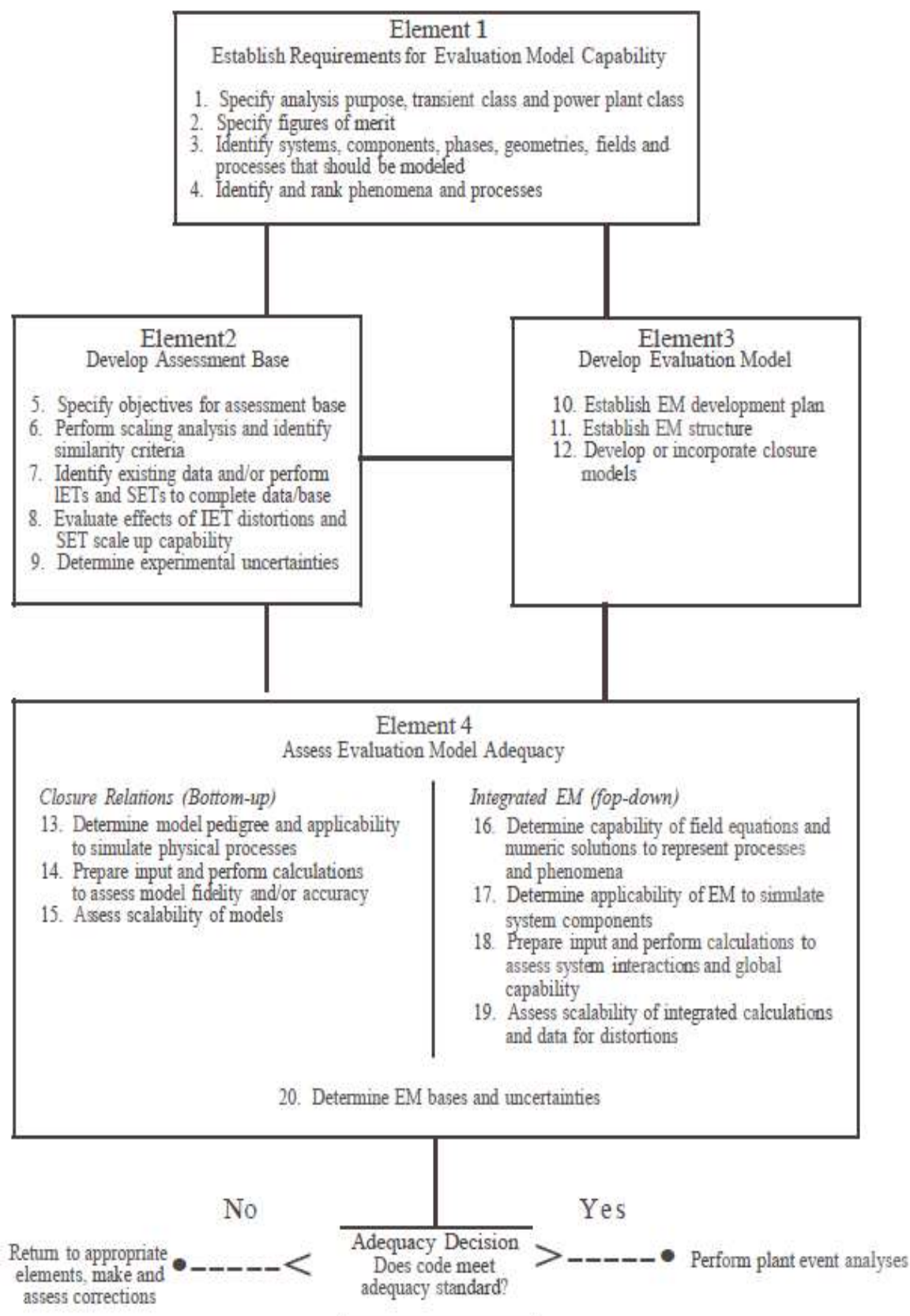
Fig. 2-4 – The EMDAP process (USNRC 2005).
