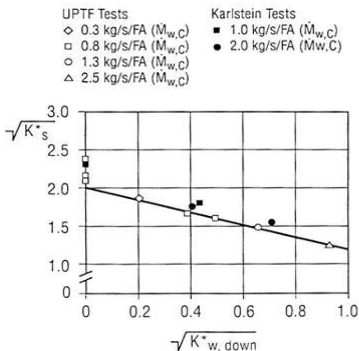
Fig. 4-11 – Counter-current flow of saturated steam and water at the tie plate for homogeneous-flow conditions.
