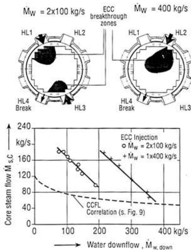
Fig. 4-12 – Counter-current flow of steam and saturated water injected into hot leg.
