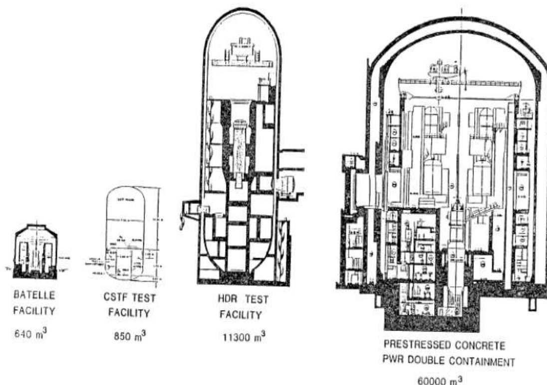
Fig. 3-4 - Comparison of test facilities with pre-stressed concrete PWR double containment, OECD/NEA/CSNI, 1989a.
