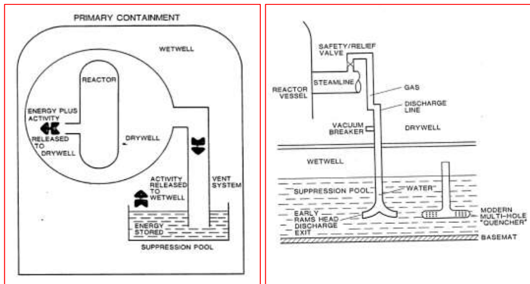
Fig. 3-5 – Left: Schematic of essential features of a pressure-suppression containment; Right: Typical Safety/relief valve-discharge line, OECD/NEA/CSNI, 1986 .
