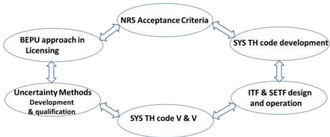
Fig. 4-18 – An overview of the Accident Analysis process in NRS.
