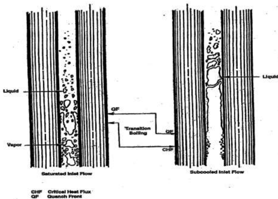
Fig. 2-2 – Qualitative reflood flow regimes at different sub-cooling (high on the right side) and flow velocity (low on the left side).
