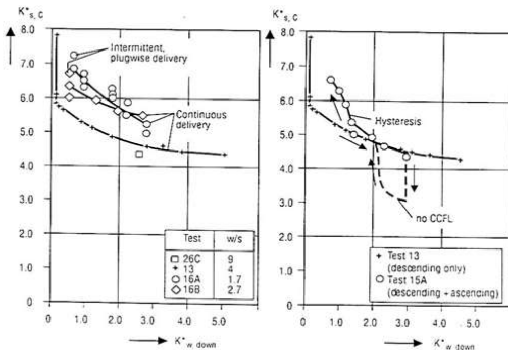
Fig. 4-13 – Counter-current flow of two-phase up-flow and subcooled water down-flow during hot leg ECC injection.
