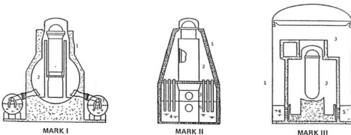
Fig. 3-6 – GE pressure suppression system design, OECD/NEA/CSNI, 1986 . (1 = primary containment; 2 = dry-well; 3 = wet-well; 4 = PSP; 5 = vent system)
