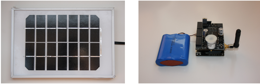
Fig. 1: Our solar energy harvesting system: The solar module KL-SUN3W (on the left) and the Waspote platform (on the right).
