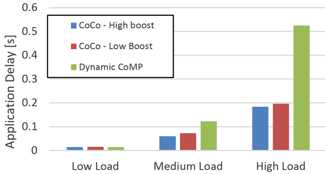
Fig. 4. Application delay with CoCo and dynamic CoMP
