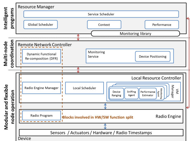
Fig. 2. Functional architecture for context and content-centric 5G platforms
