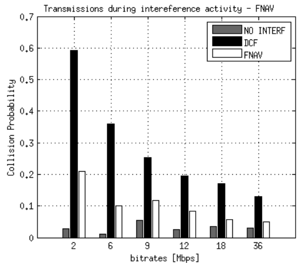
Fig. 3. Collision probability for different values of the bit rate
