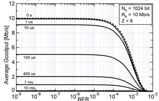
Fig. 7: \overline{GP} vs. BER for a link with ARQ at different values of T_w
