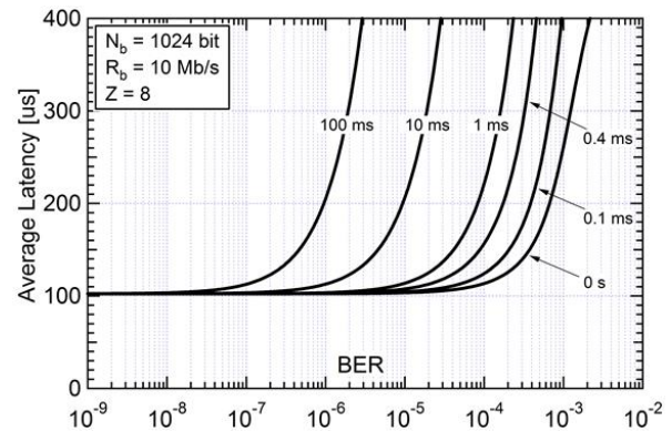
Fig. 8: \overline{T}_{succ} vs. BER for a link with ARQ at different T_w values
