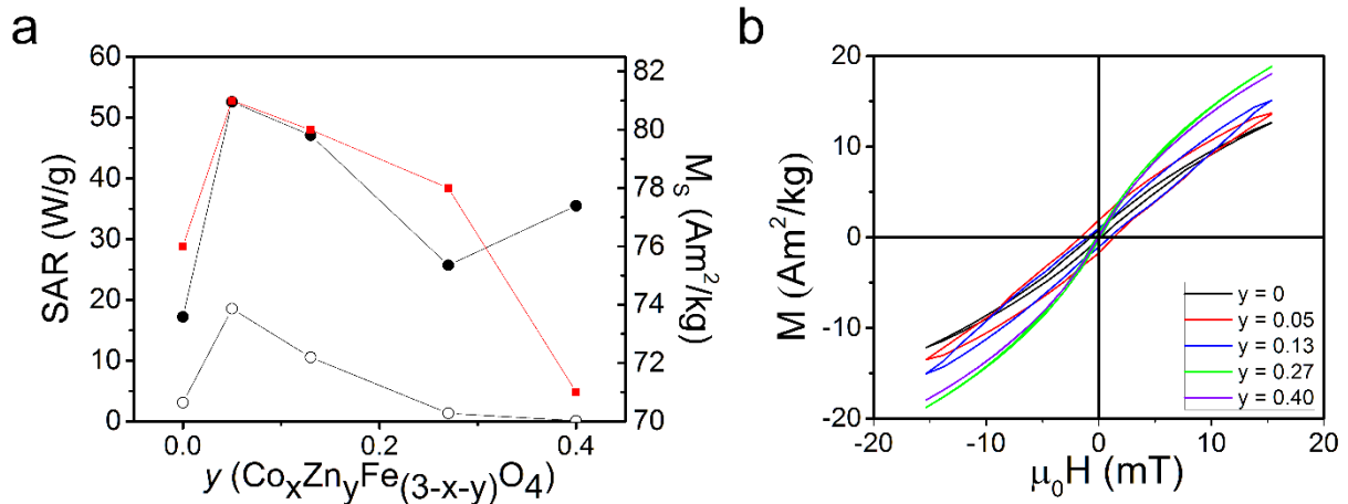
Figure 7. a) SAR values of \text{Co}_x\text{Zn}_y\text{Fe}_{(3-x-y)}\text{O}_4 NPs as a function of Zn-content y experimentally measured (full circles) and evaluated by the minor loop area multiplied by the operating frequency, SAR hl (empty circles); the M_S values (full squares) are reported for comparison; b) Minor loop recorded at 300K with H_{max} = 12 kA/m ( \mu_0 H_{max} = 15.3 mT).
