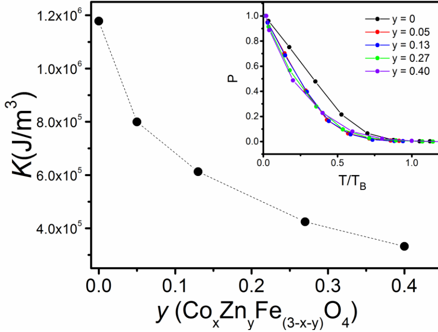
Figure 5. Anisotropy constant K of \text{Co}_x\text{Zn}_y\text{Fe}_{(3-x-y)}\text{O}_4 NPs as a function of Zn-content y . In the inset, dependence of the product P=H_C \cdot M_S normalized to 5 K value on the reduced temperature T/T_B . For \text{CoZnFe05} T_B was extrapolated to 350 K from the H_C(T) curve, as H_C(T \rightarrow T_B) \rightarrow 0 .
