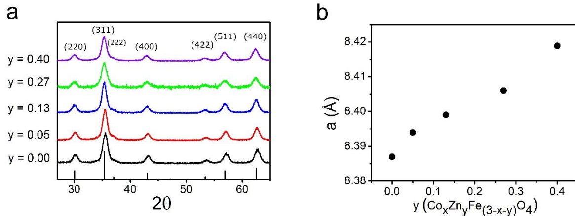
Figure 2. a) X-ray diffraction patterns of \text{Co}_x\text{Zn}_y\text{Fe}_{3-(x+y)}\text{O}_4 NPs compared to the reference pattern of cobalt ferrite (black bars); b) Lattice parameter dependence on the Zn-content, y (error is within 0.003 Å).
