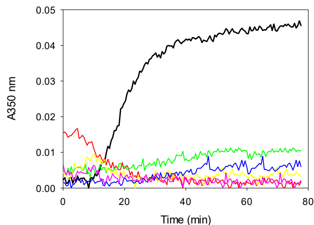
Figure 6. Turbidity time course for the assembly of 25 \mu\text{M} tubulin at 37 ^{\circ}\text{C} in the presence of 27.5 \mu\text{M} of the compounds followed at 350 nm. Black line (DMSO, vehicle), green line ( 6d ), yellow line ( 6f ), pink line ( 6h ), red line ( 6m ), blue line ( 6n ).
