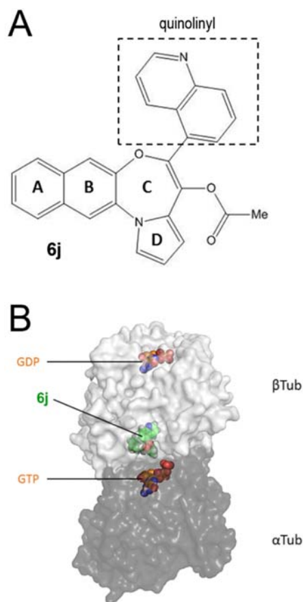
Figure 8. X-ray crystallographic studies on 6j. (A) Chemical structure of 6j. The A, B, C and D cycles are part of the naphtho-pyrrolo-benzoxazepine moiety. The quinolinyl moiety is
