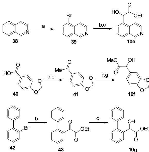
Scheme 5. Synthesis of \alpha -hydroxyesters 10e-g . a
