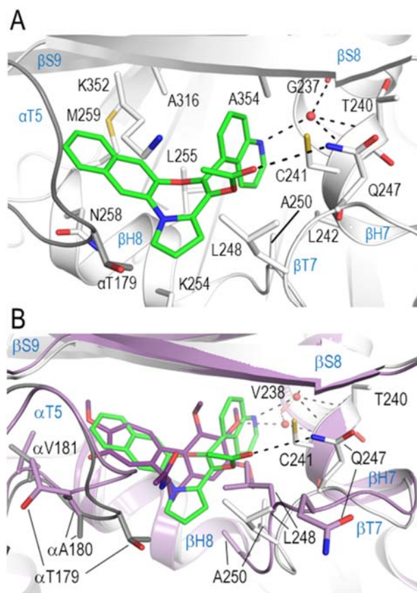
Figure 9. Detailed interactions between tubulin and 6j . (A) Close-up view of the interaction mode between 6j and tubulin. 6j and interacting tubulin residues are shown in green and grey sticks representation, respectively. Tubulin secondary structural elements are labeled with blue letters. (B) Superimposition of the 6j -tubulin ( 6j in green sticks) and 4 -tubulin (PDB ID 4O2B; 4 in violet sticks) complex structures. In both figures, oxygen, nitrogen and sulfur atoms are colored in red, blue and yellow, respectively. Hydrogen bonds are represented by black dotted lines, and the water molecules are displayed as a red sphere. Tubulin secondary structural elements are labeled with blue letters.
