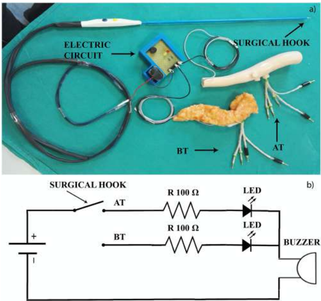
Fig. 6. Circuit for acoustic functionality: a) Simple electric circuit signaling the damages to AT and/or BT walls b) Equivalent electric scheme.
