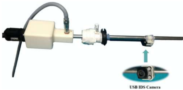
Fig. 7. Laparoscope equipped with the block and the USB camera.
