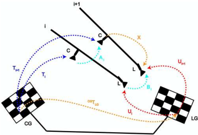
Fig. 9. Set-up of hand-eye calibration.
