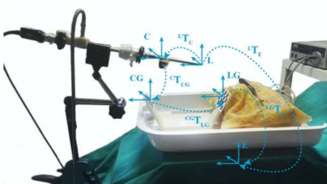
Fig. 8. Transformation (represented by dashed line) and Coordinate frames.
