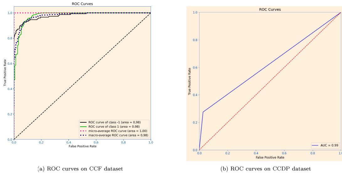
Fig. 12. ROC curves of proposed model on CCF & CCDP dataset.
