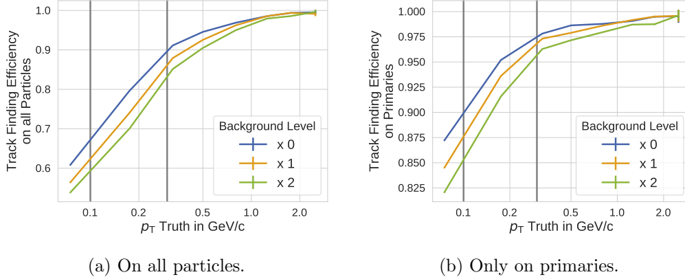
Figure 14: Track finding efficiency calculated for simulated \Upsilon(4S) events with different levels of beam-induced background relative to the expected level. Figure 14a is calculated on all trackable simulated particles, whereas Figure 14b only takes into account trackable particles from the primary interaction. The gray vertical lines indicate the typical transverse momentum of particles only trackable in the VXD (below left line) and with high efficiency in the CDC (above right line).
