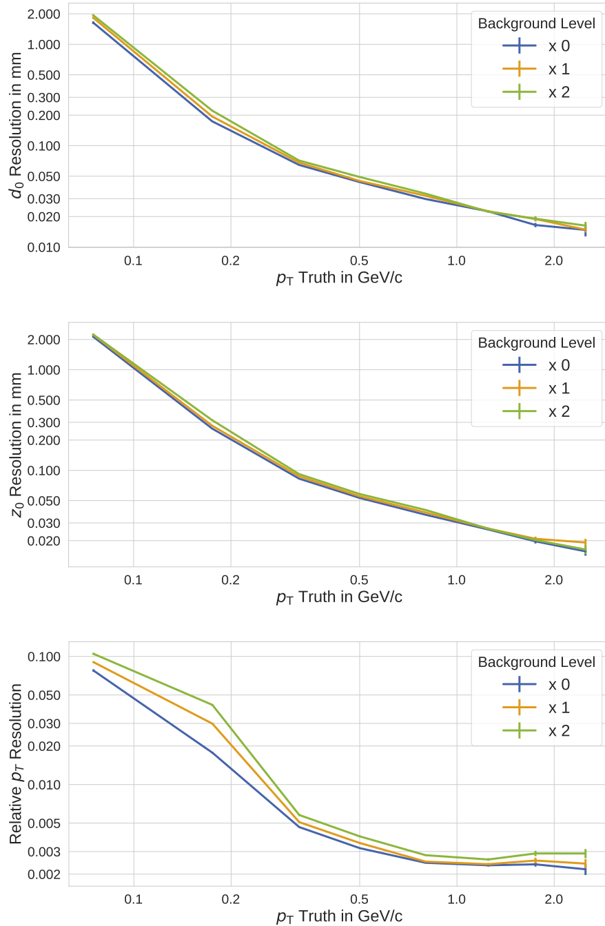
Figure 17: Resolutions for typical simulated \Upsilon(4S) events with different levels of beam-induced background. As most of the simulated final state particles are pions, only the results of this fit hypothesis are shown.
