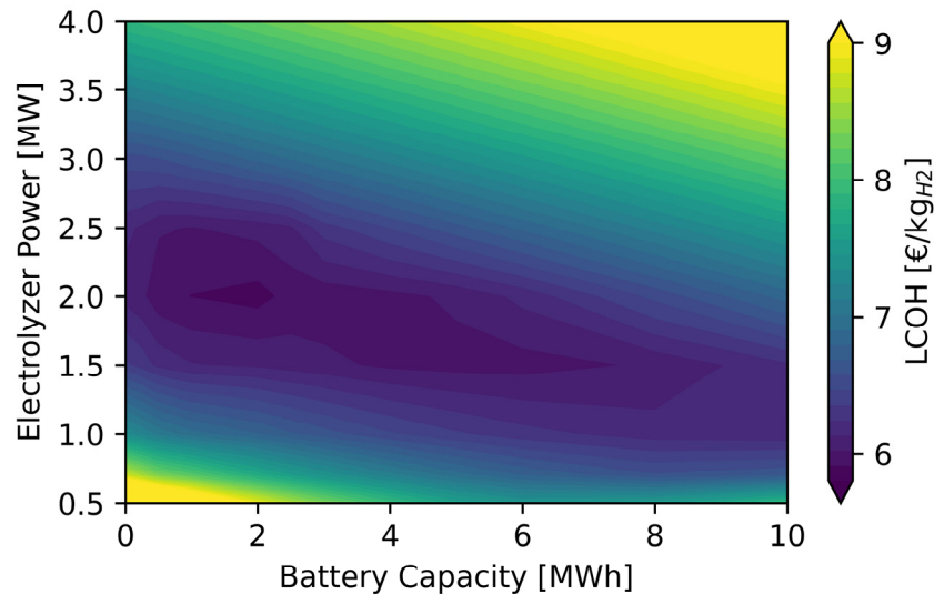
Figure 7. LCOH heatmap varying battery capacity and electrolyzer power.
