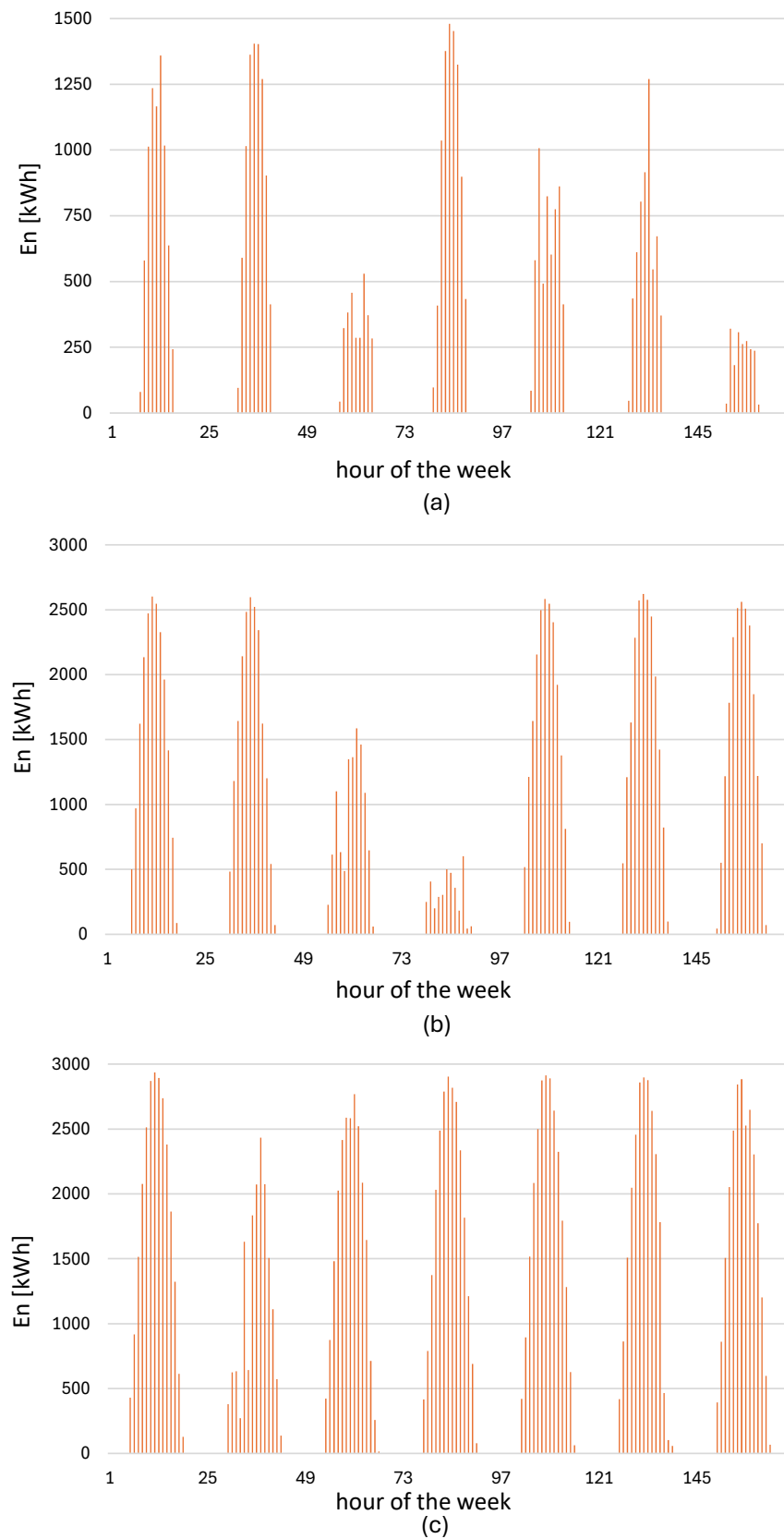
Figure 3. Energy generated by the PV plant in three weeks in January (a), April (b), and July (c).
