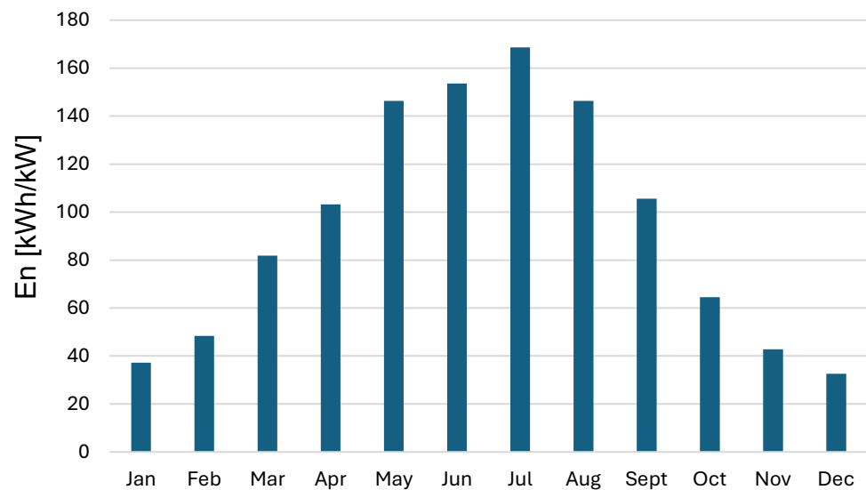
Figure 5. Specific energy produced monthly by the PV plant.
