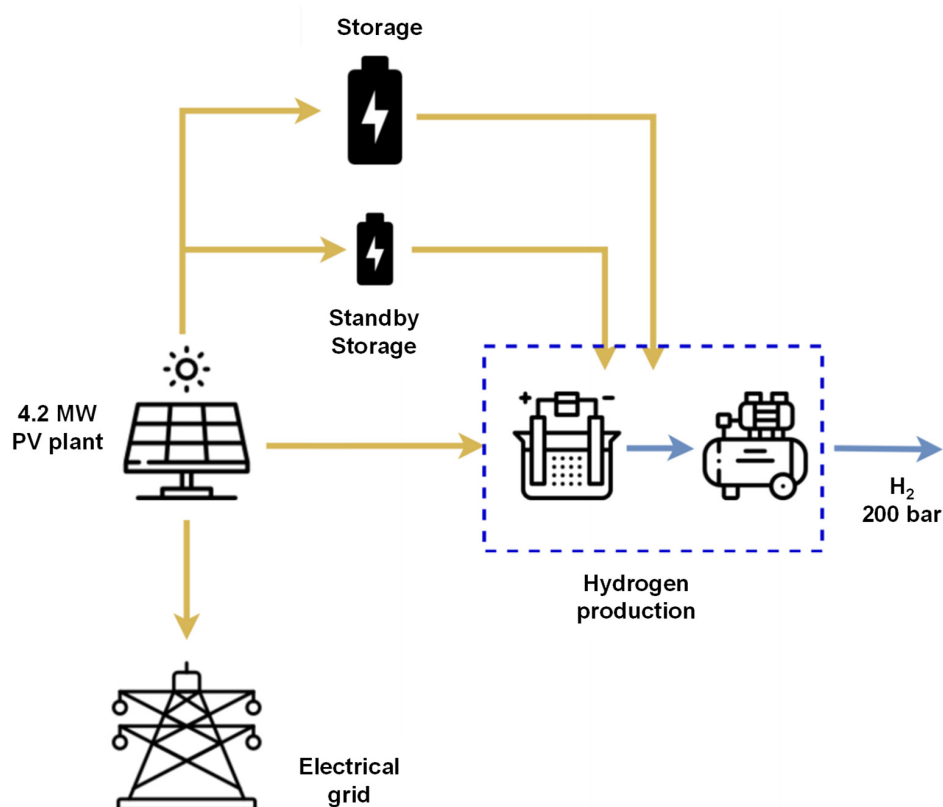
Figure 2. Schematic representation of a scalable and flexible plant configuration integrating hydrogen generation and compression, and electrical power generation.
