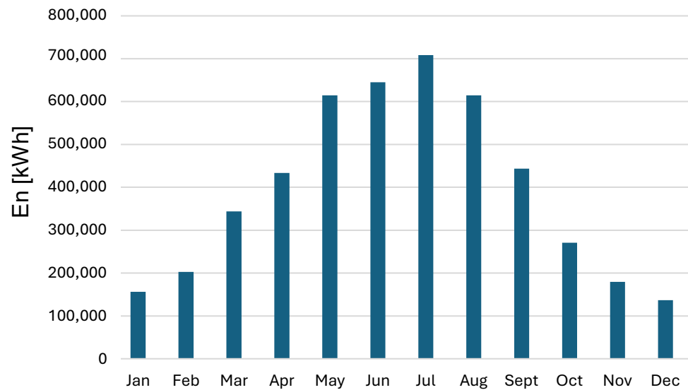
Figure 4. Energy generated by the PV plant for each month.
