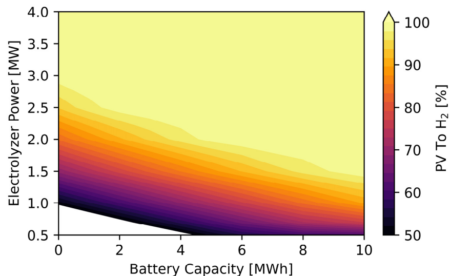
Figure 8. Percentage of PV energy to hydrogen production heatmap varying battery capacity and electrolyzer power.
