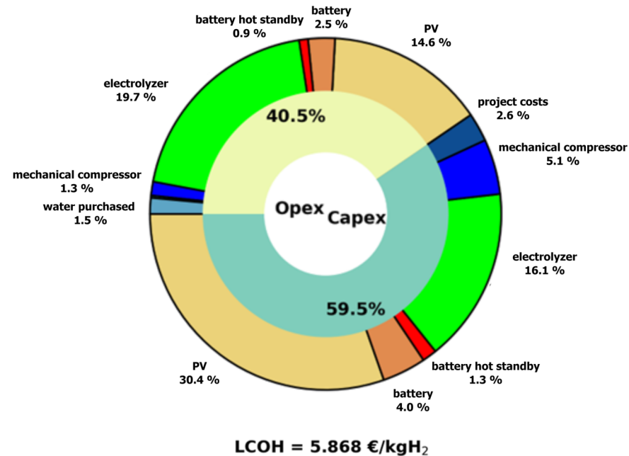
Figure 9. Technologies contributions to Levelized Cost of Hydrogen.
