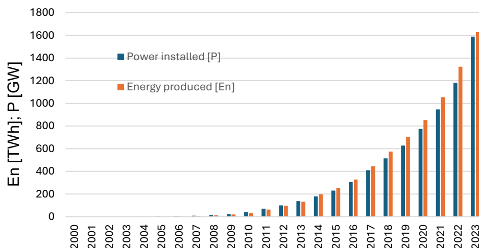
Figure 1. Global photovoltaic (PV) installations: trends in installed capacity (GW) and energy generation (TWh) in the current century.
