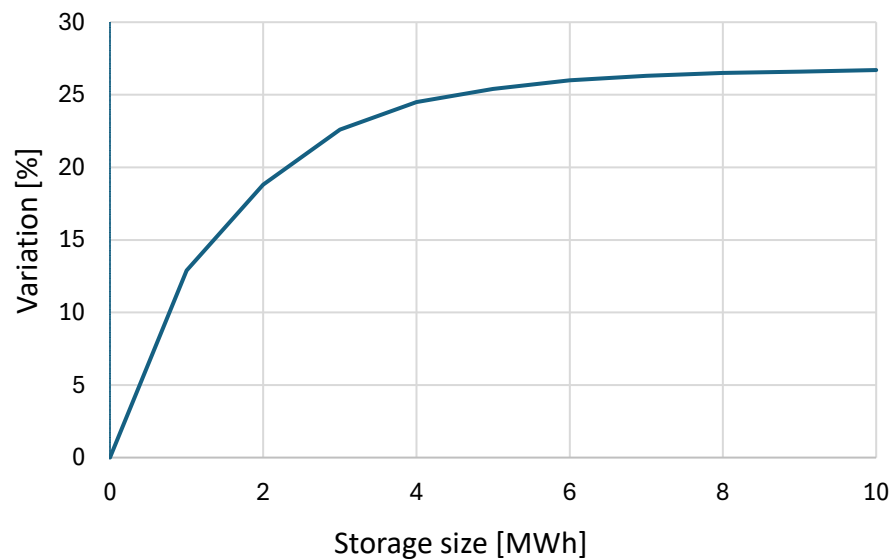
Figure 6. Increase in hydrogen production with the increase in the size of the storage.
