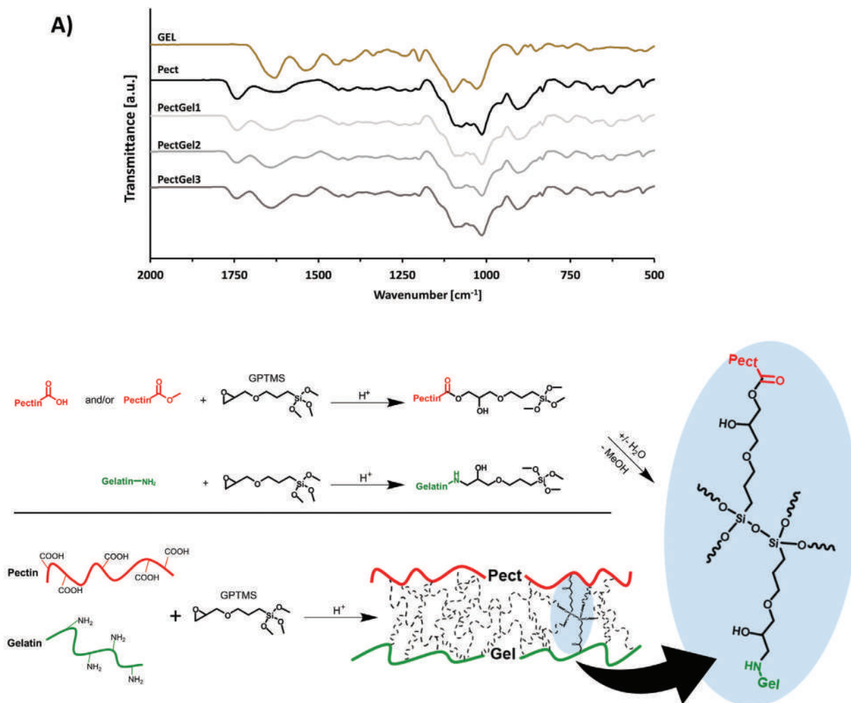
Figure 1. A) ATR-IR spectra of PectGel1, PectGel2 and PectGel3, Pect and GEL. B) Hypothetical crosslinking reaction mechanism in an aqueous environment; in an acidic environment, as generated by pectin, the GPTMS epoxide ring is opened and the resulting hydroxyl groups react with the carbonyl groups of pectin. [3] Concomitantly, an acid-catalyzed epoxide ring-opening occurs by primary amines on gelatin. [28,29] The two reactions lead to GPTMS residues linked by esters to pectin and linked by secondary amines to gelatin. Subsequently, in an aqueous environment, hydrolysis of the trimethoxysilane groups occurs (expulsion of methanol) followed by a condensation reaction forming Si-O-Si-linkages between polymer chains. [30] It must be noted that the reactions linking GPTMS to both polymers occur simultaneously in our system and are likely to compete. Which reaction is dominant and whether one of the reaction products is formed in majority is still under investigation.
