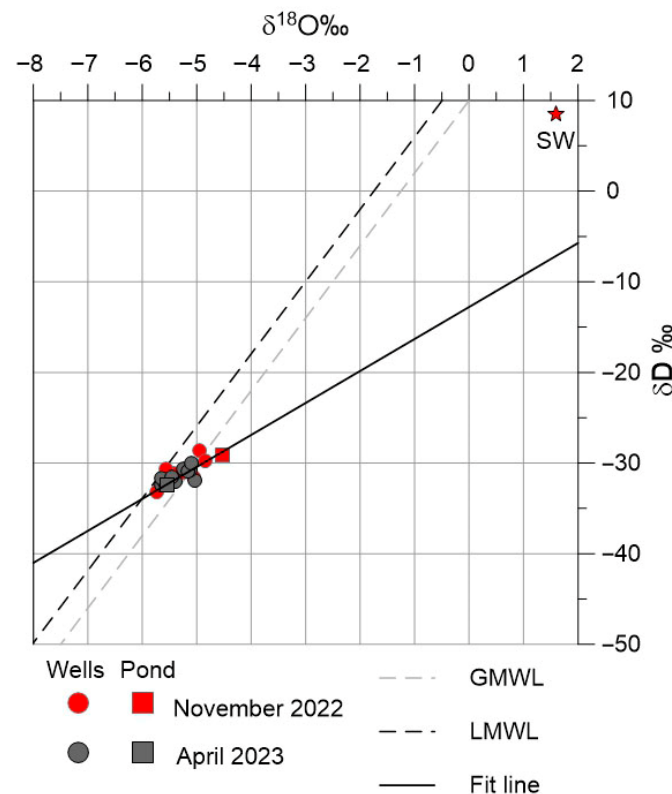
Figure 12. \delta D versus \delta^{18}O relationship for groundwater in the study area.
