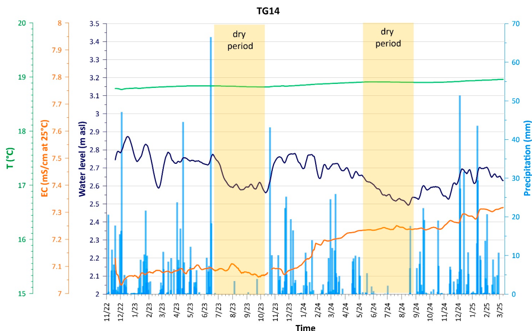
Figure 7. One-week moving averages of temperature (T), electrical conductivity (EC), and water levels, compared to daily precipitation in well TG14.
