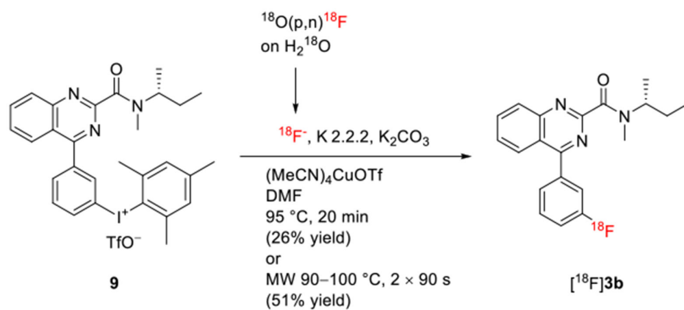
Scheme 6. Radiosynthesis of [^{18}\text{F}]\mathbf{3b}
