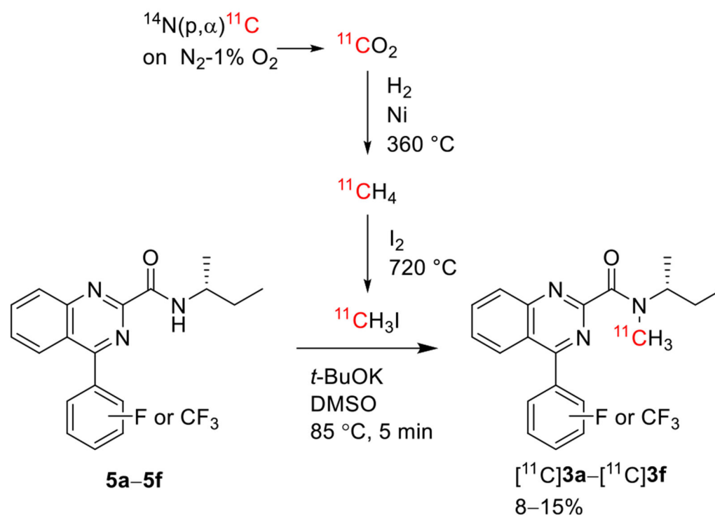
Scheme 4. Radiosyntheses of Radioligands [ ^{11}\text{C} ]3a–[ ^{11}\text{C} ]3f
