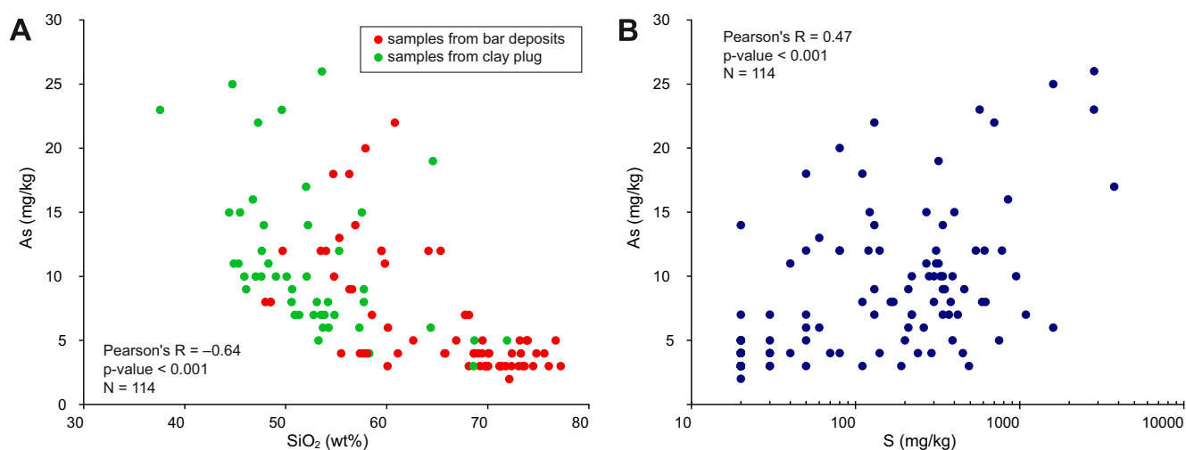
Fig. 7. Scatterplots showing relationships between sediment As concentrations and \text{SiO}_2 (A) and between As and S (B).
