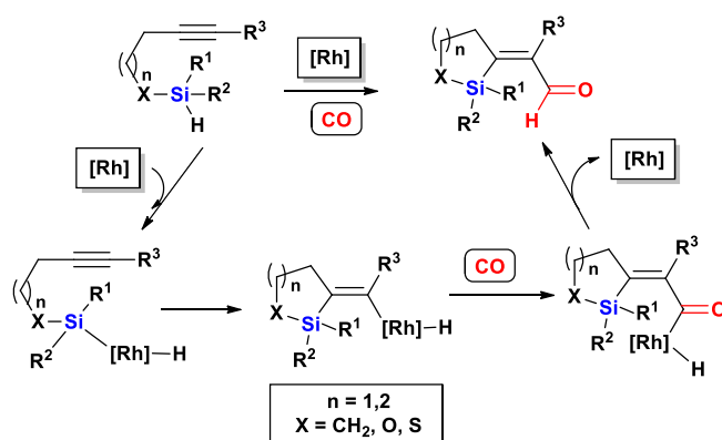
Scheme 4. General mechanism for intramolecular silylformylation reactions.
