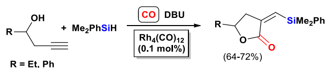
Scheme 41. Heteroatom-promoted SiCAC of homopropargyl alcohols: synthesis of \gamma -lactones.
