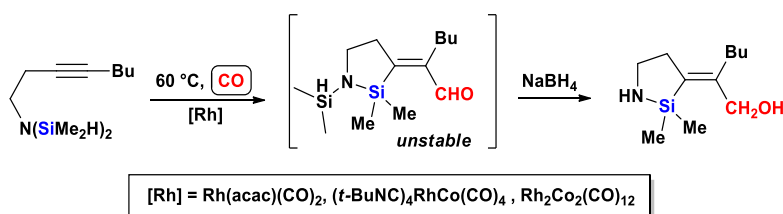
Scheme 7. Intramolecular silylformylation/desilylation of 1-bis(dimethylsilylamino)-3-octyne.
