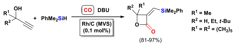
Scheme 43. Heteroatom-promoted SiCAC of 3-dialkylpropargyl alcohols catalyzed by Rh/C (MVS).
