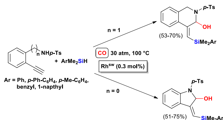
Scheme 57. Synthesis of tosylindolinols and tosyltetrahydroisoquinolinols via heteroatom-promoted SiCAC with several \text{ArMe}_2\text{SiH} .
