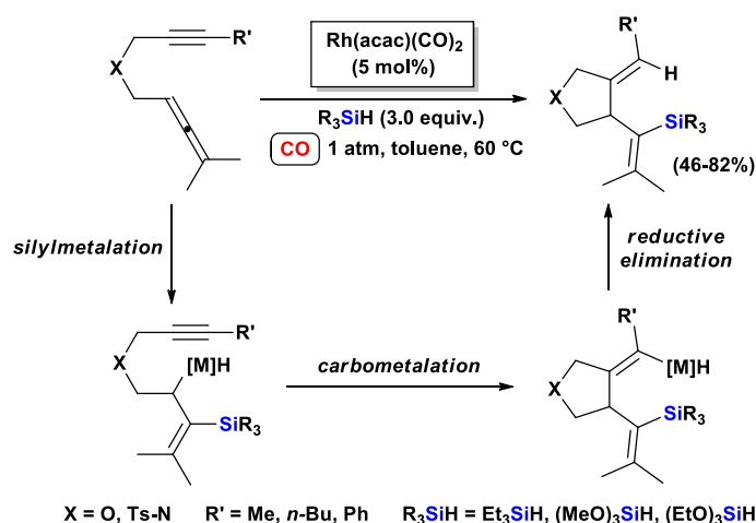
Scheme 30. Standard SiCAC of propargyl homoallenyl ethers and amines under atmospheric CO pressure: synthesis of cyclic (tetrahydrofuran or pyrrolidine) 1,4-dienes.
