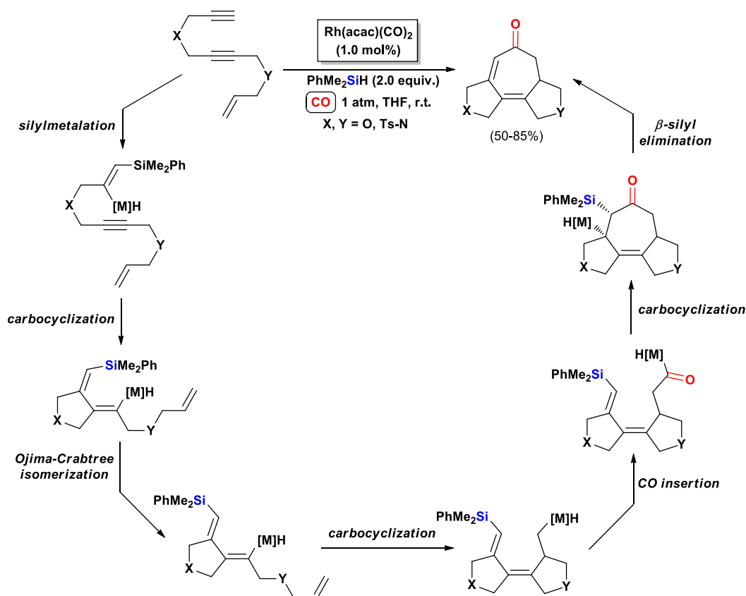
Scheme 31. First investigation of cascade SiCAC of enediyne: the proposed reaction mechanism involved three sequential carbocyclization steps, hence the name “ cascade SiCAC”.
