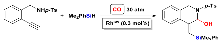
Scheme 56. Heteroatom-promoted SiCAC applied to the synthesis of tosyltetrahydroisoquinolinols.
