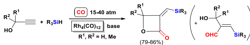
Scheme 34. First example of heteroatom-promoted silylcarboxylation of ethynyl alcohols.
