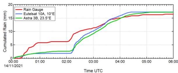
Figure 6. Cumulated rain provided by a MSRS and a TBRG in Pisa, Italy.
