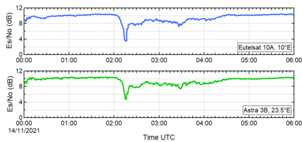
Figure 5. Sample records of E_s/N_0 measured in Pisa, Italy, from a MSRS with a MSmartLNB receiver: Eutelsat 10A at 10°E (top); Astra 3B at 23.5°E (bottom).
