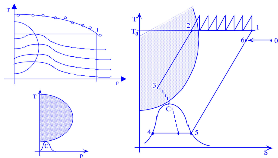
Figure 2. Schematic representation of hydrogen compression in gaseous or liquid form in a T-S diagram.
