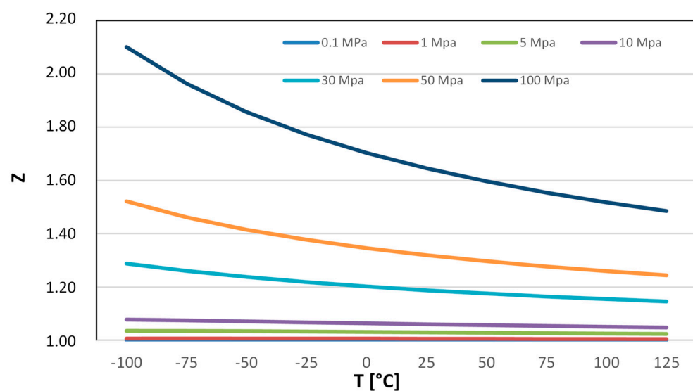
Figure A2. Hydrogen compressibility (Z) at different temperatures and pressures.
