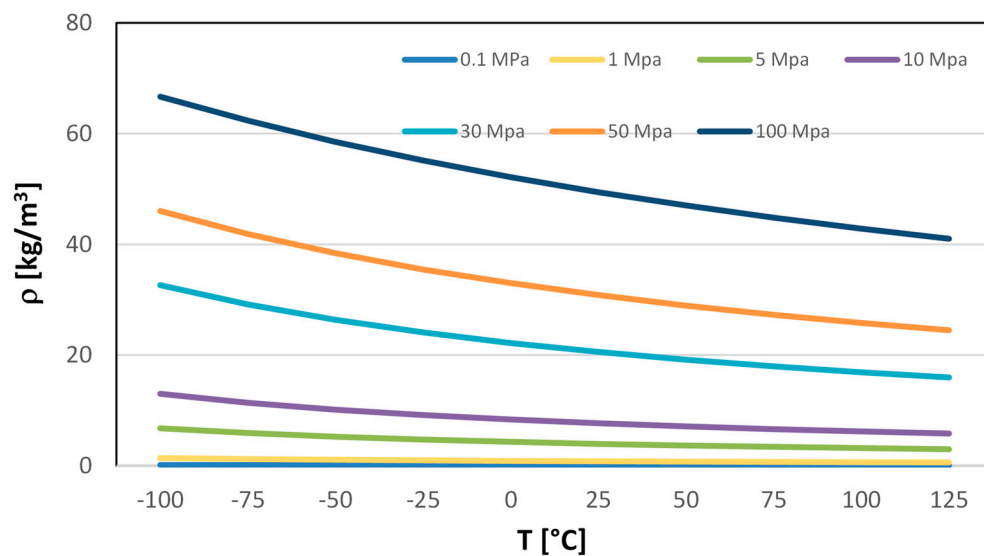
Figure A1. Hydrogen density as a function of temperature and pressure.
