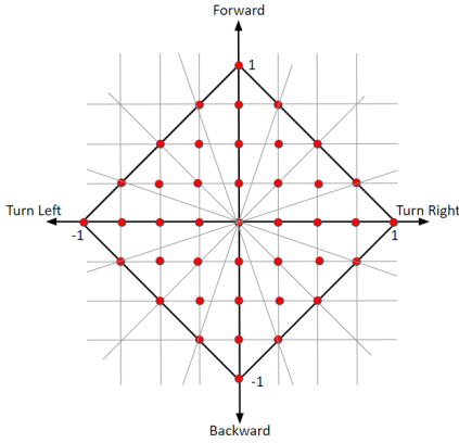
Figure 2: Continuous user and discretised Agent joysticks.
