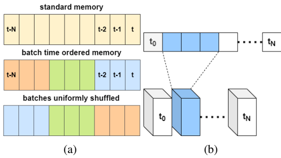
Figure 3: Memory management: (a) grouped sequential memory; (b) samples in another dimension.
