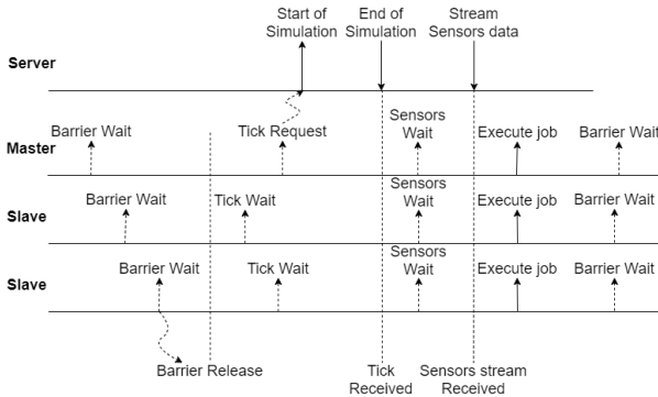
Figure 4: Synchronisation mechanism among clients and server.
