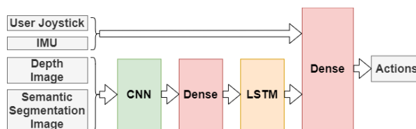
Figure 6: Neural network components overview.
