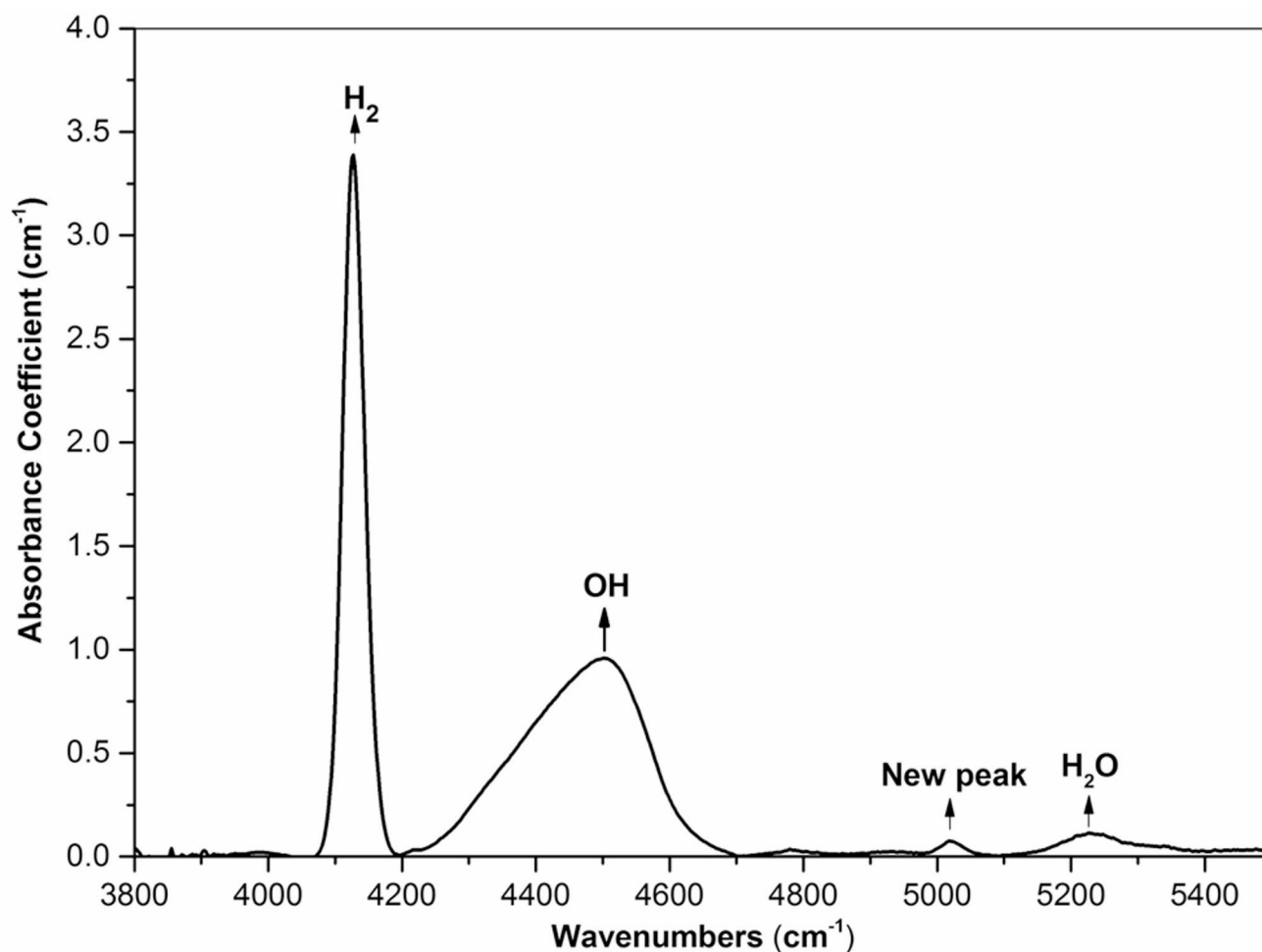
Fig. 2 Background-corrected infrared spectrum of sample AMPC15 showing the main absorption bands and the “new peak” assigned to a combination mode of molecular H_2
