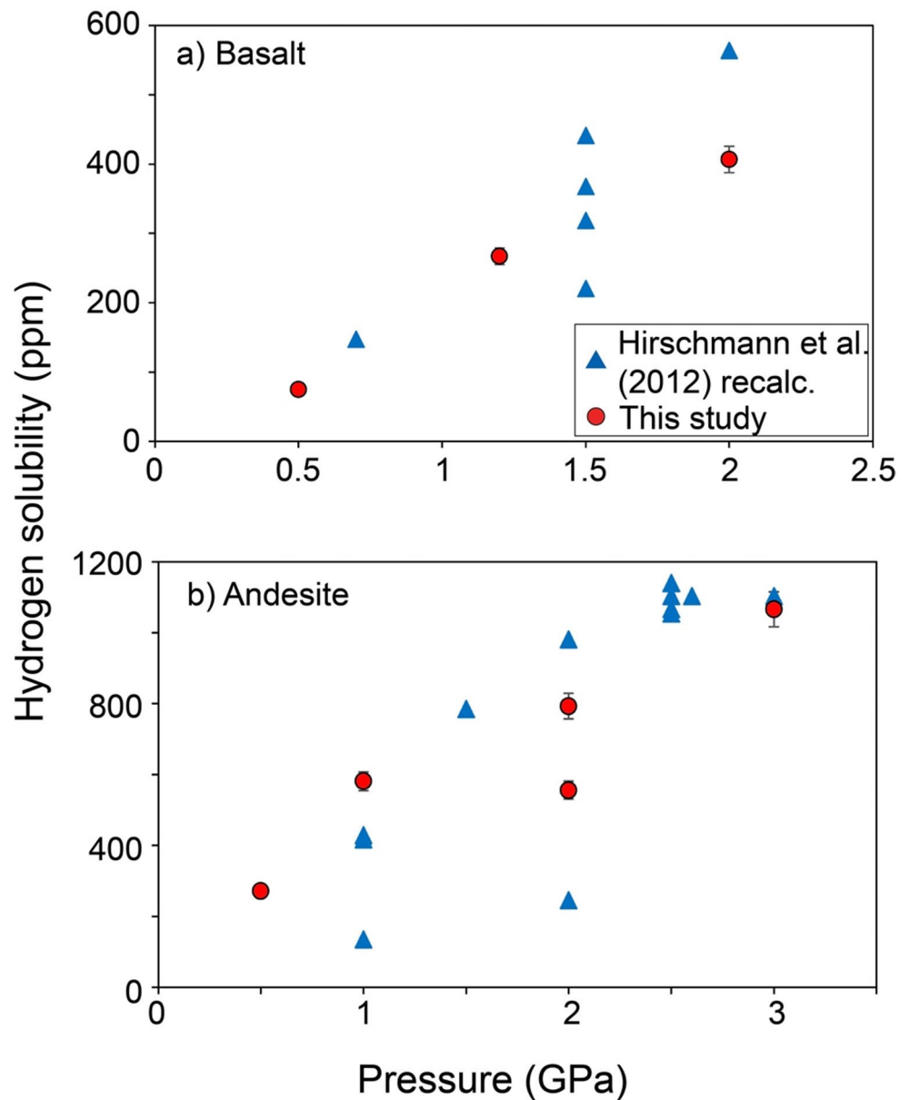
Fig. 8 Comparison of the results of the current study with that of Hirschmann et al. (2012) on H_2 solubility in basaltic and andesitic melt as a function of pressure. Only experiments carried out at Fe-FeO- H_2O buffer conditions are shown. The data from Hirschmann et al. (2012) are recalculated using the infrared extinction coefficient obtained in the current study, which reduces the values by one order of magnitude as compared to those previously reported. The basalt and andesite experiments of the current study were all performed at 1400 °C, like most of those of Hirschmann et al. (2012). The latter dataset also includes two basalt experiments at 1450 °C and two andesite experiments at 1500 °C. For the definition of the error bars see Table 2. No estimates of error are available for the original solubility data of Hirschmann et al. (2012)
