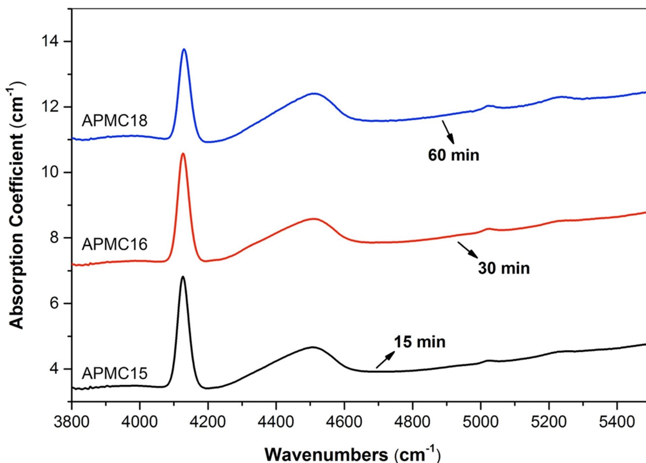
Fig. 1 Infrared spectra of three H 2 -bearing haplogranitic glasses produced at 1.5 GPa, 1200 °C and Fe-FeO-H 2 O buffer conditions with different run durations
