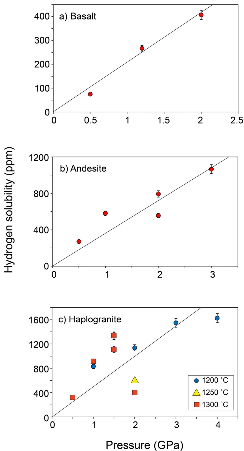
Fig. 7 H_2 solubility in basaltic, andesitic, and haplogranitic melt at Fe-FeO- H_2O buffer conditions as a function of pressure. The basalt and andesite experiments were all carried out at 1400 °C. Shown are also linear regression curves for all data of the form c_{H_2} = a_{Henry} P , with a_{Henry} = (206 \pm 10) ppm/GPa for basalt, (362 \pm 35) ppm/GPa for andesite, and (500 \pm 62) ppm/GPa for haplogranite. For the definition of the error bars see Table 2
