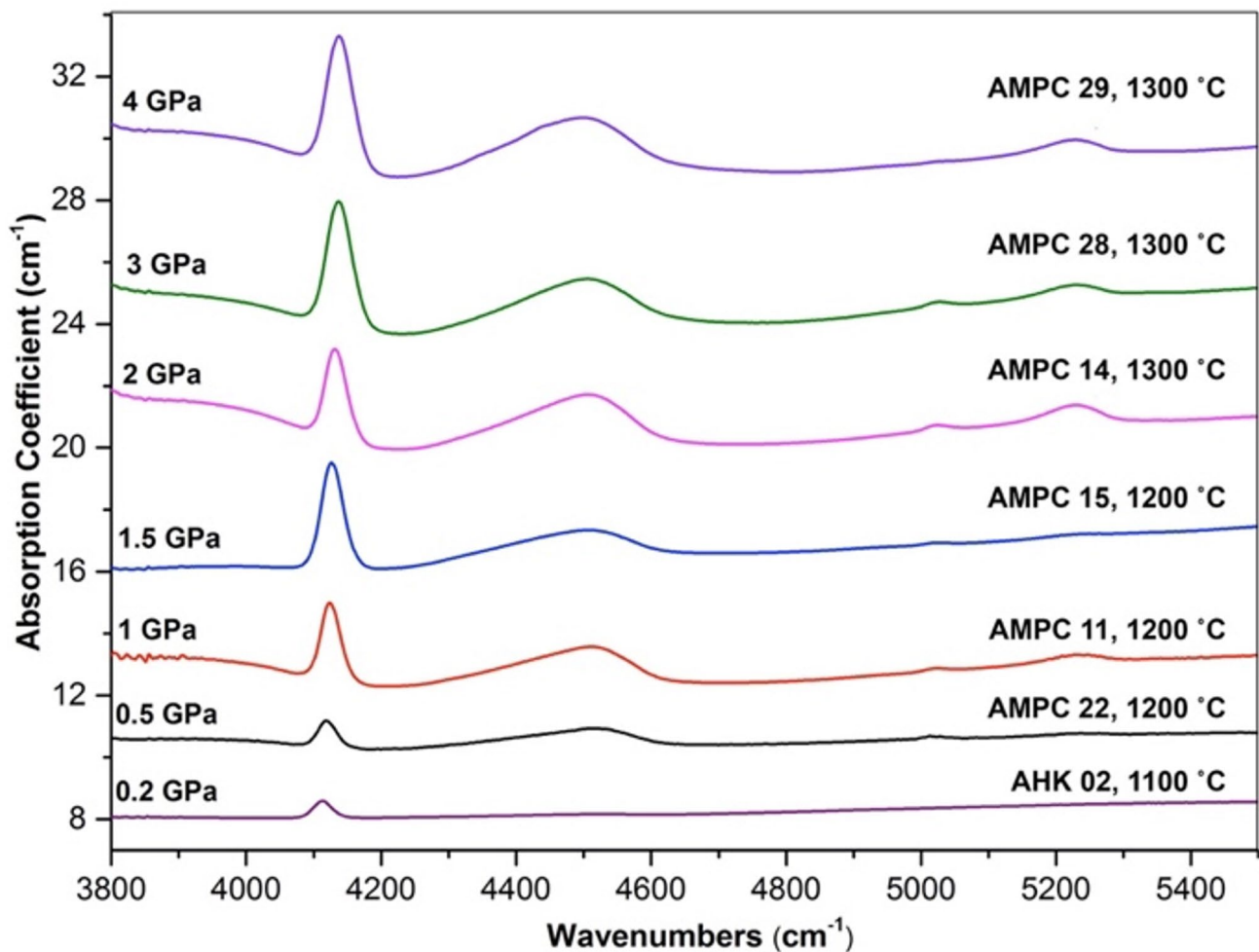
Fig. 6 Effect of pressure on H_2 solubility in haplogranitic melt, as seen in the infrared spectra. Sample AHK02 was equilibrated with pure H_2 gas, the others were in equilibrium with the Fe-FeO- H_2O buffer
