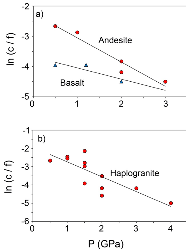
Fig. 9 Thermodynamic treatment of H 2 solubility in silicate melts. Shown is a plot of \ln(c/f) versus pressure, where c is H 2 concentration in the melt in ppm by weight and f is hydrogen fugacity. The data for basalt and andesite are for 1400 °C, the haplogranite data for 1200 to 1300 °C. Errors due to analytical uncertainties in c are smaller than the symbols shown, but errors due to possible incomplete equilibration cannot be quantified. The regression lines shown have the form \ln(c/f) = a + b P , with a = -3.675 , b = -0.371 for basalt, a = -2.250 , b = -0.801 for andesite, and a = -1.930 , b = -0.811 for haplogranite
