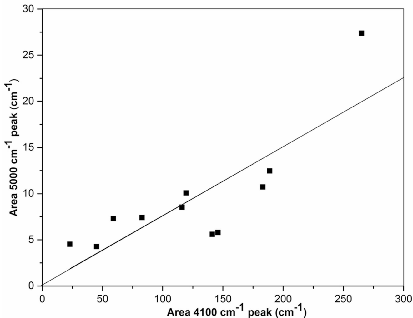
Fig. 3 Correlation between the integral intensity of the band near 5000\text{ cm}^{-1} and the main \text{H}_2 band near 4100\text{ cm}^{-1} for haplogranitic glasses
