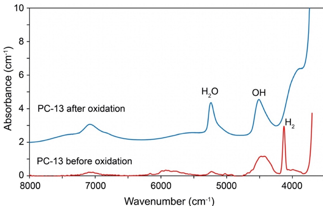
Fig. 4 Calibration of the 4100\text{ cm}^{-1} infrared band of \text{H}_2 in haplogranitic glass by oxidation with \text{O}_2 . Shown are the infrared spectra of the \text{H}_2 -saturated sample PC-13 before and after oxidation by treatment with \text{O}_2 . The prominent \text{H}_2 band at 4100\text{ cm}^{-1} in the initial sample
