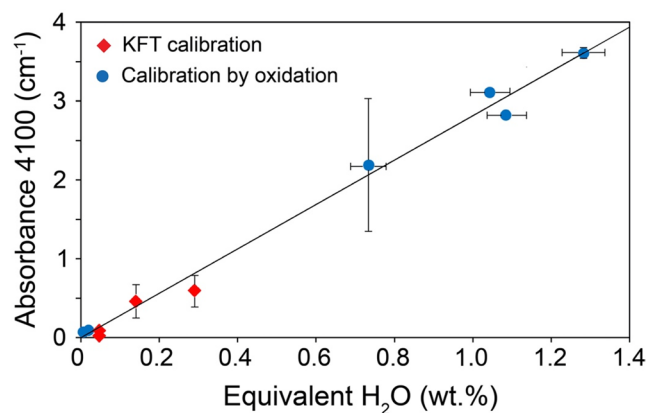
Fig. 5 Calibration of the 4100 cm -1 infrared band of H 2 in haplogranitic glass by Karl Fischer titration (KFT) and by oxidation with O 2 . The sample with the large error bar was initially inhomogeneous. Where no error bar is shown, the uncertainty is smaller than the size of the symbol. “Equivalent H 2 O” is the concentration of H 2 O (in wt%) corresponding to the equal molar concentration (in mol/liter) of H 2 in the glass. The slope of the regression line shown is 2.800 ± 0.064 (R 2 =0.9977), which corresponds to an extinction coefficient of (2.12 ± 0.05) liter mol -1 cm -1
